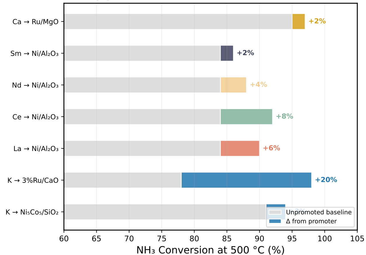
(a) Promoter Effect on NH 3 Conversion
