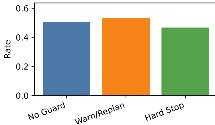
Post-trigger repetition
