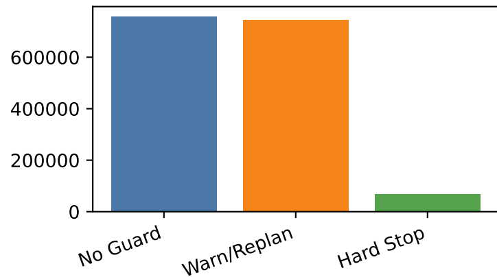
Mean tokens
