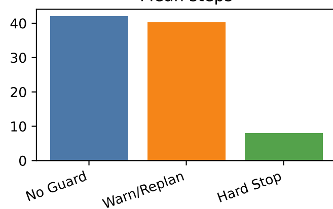
Mean steps
