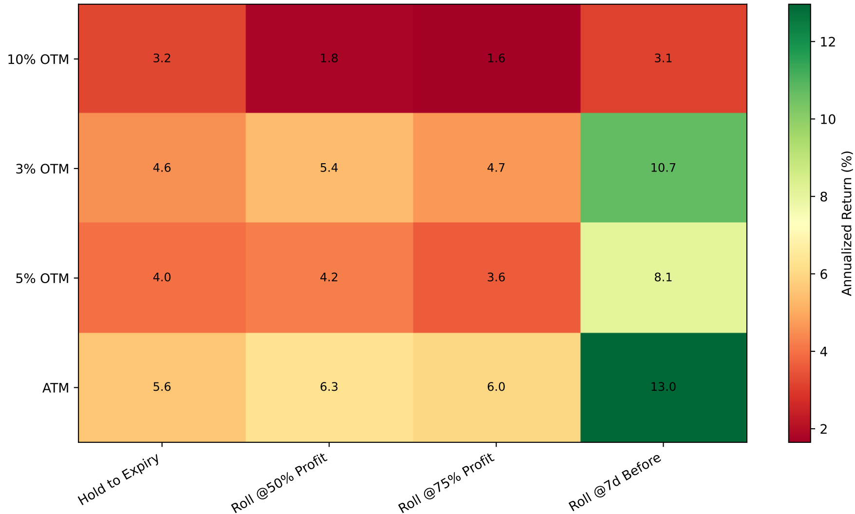
IWM: Avg Annualized Return (%) by Strike × Roll
