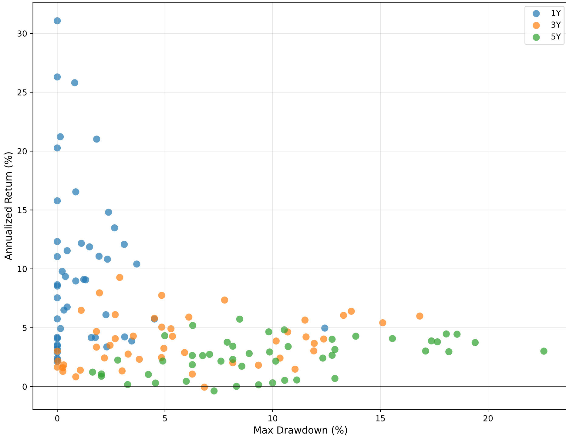
IWM: Return vs Drawdown (All Configs)
