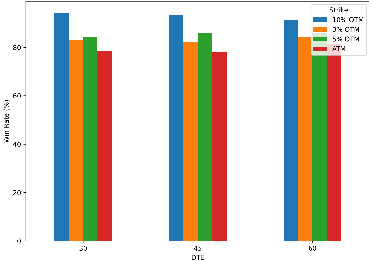
IWM: Win Rate by DTE & Strike
