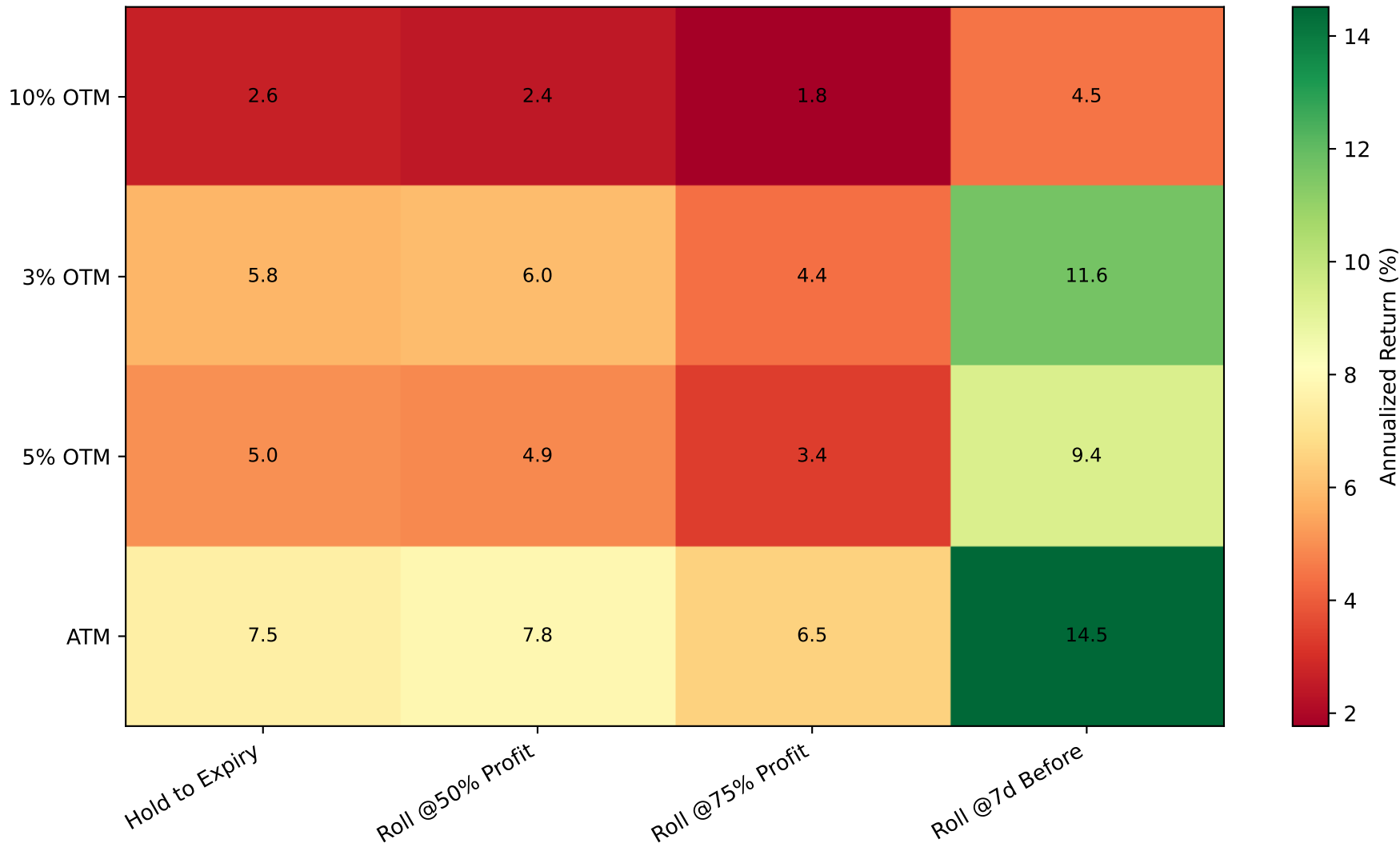
JPM: Avg Annualized Return (%) by Strike × Roll
