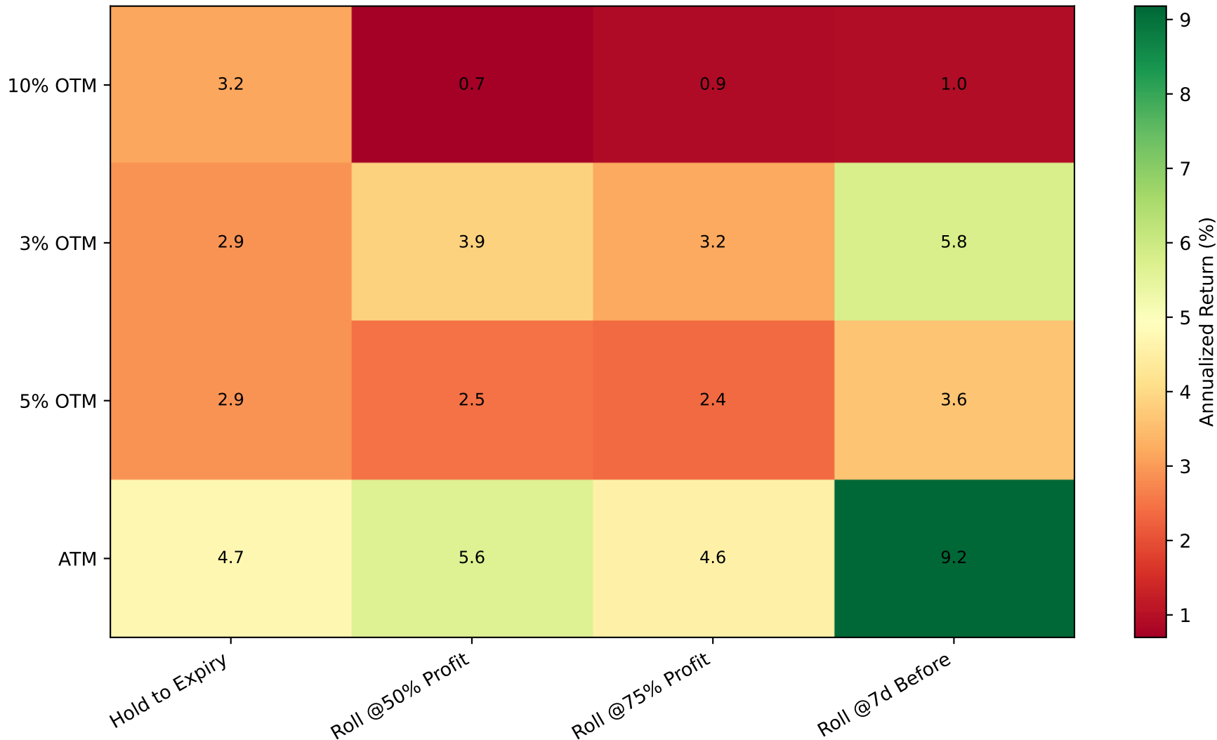
SPYM: Avg Annualized Return (%) by Strike × Roll
