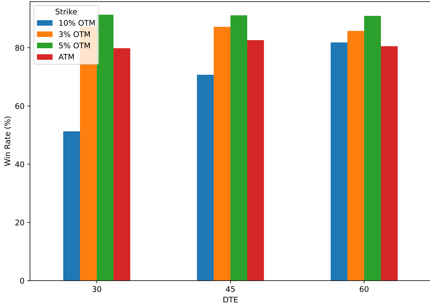
SPYM: Win Rate by DTE & Strike
