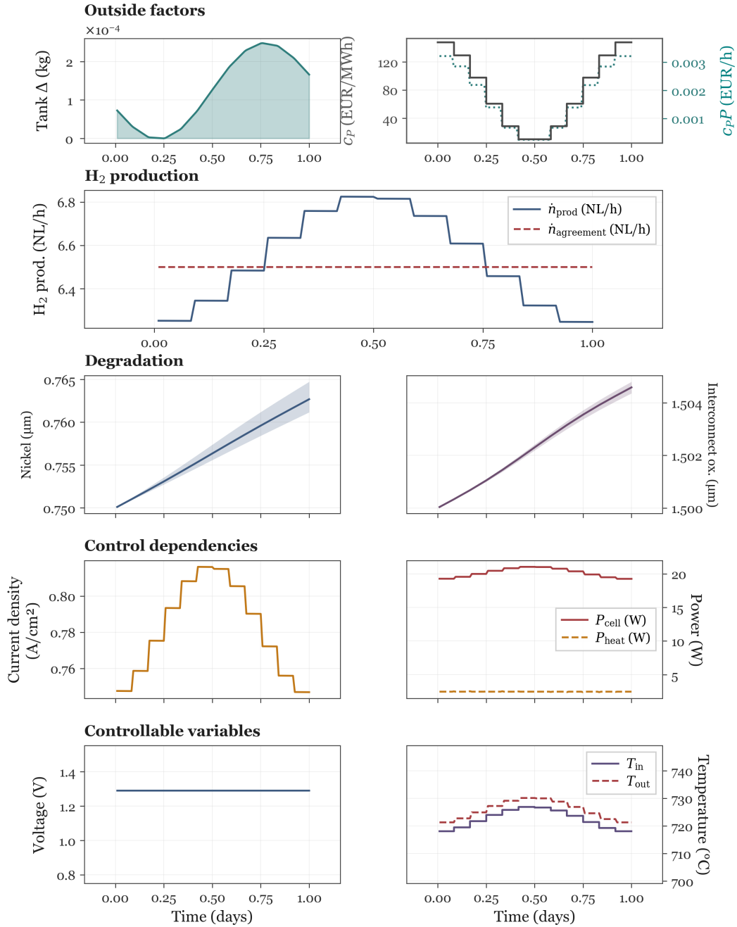
Figure 5.6: 24-hour cyclic optimum under a diurnal power price ( N_t = 12 ; table 5.4). Fixed U \approx 1.289 V ( w_U = 0.1 ); T_{\text{in}} is modulated ( w_T = 10^{-5} ) to shift production toward low-price midday segments ( c_P and c_P P in Outside factors ). Peak \dot{n}_{\text{H}_2, \text{prod}} \approx 6.8 NL/h versus \approx 6.2 NL/h overnight; the agreement rate 6.5 NL/h is met on average via cyclic tank use ( \kappa_{\text{sell}} = 0 ). Running revenue \Phi \approx 0.062 EUR, terminal salvation \Psi \approx 1.91 EUR.
