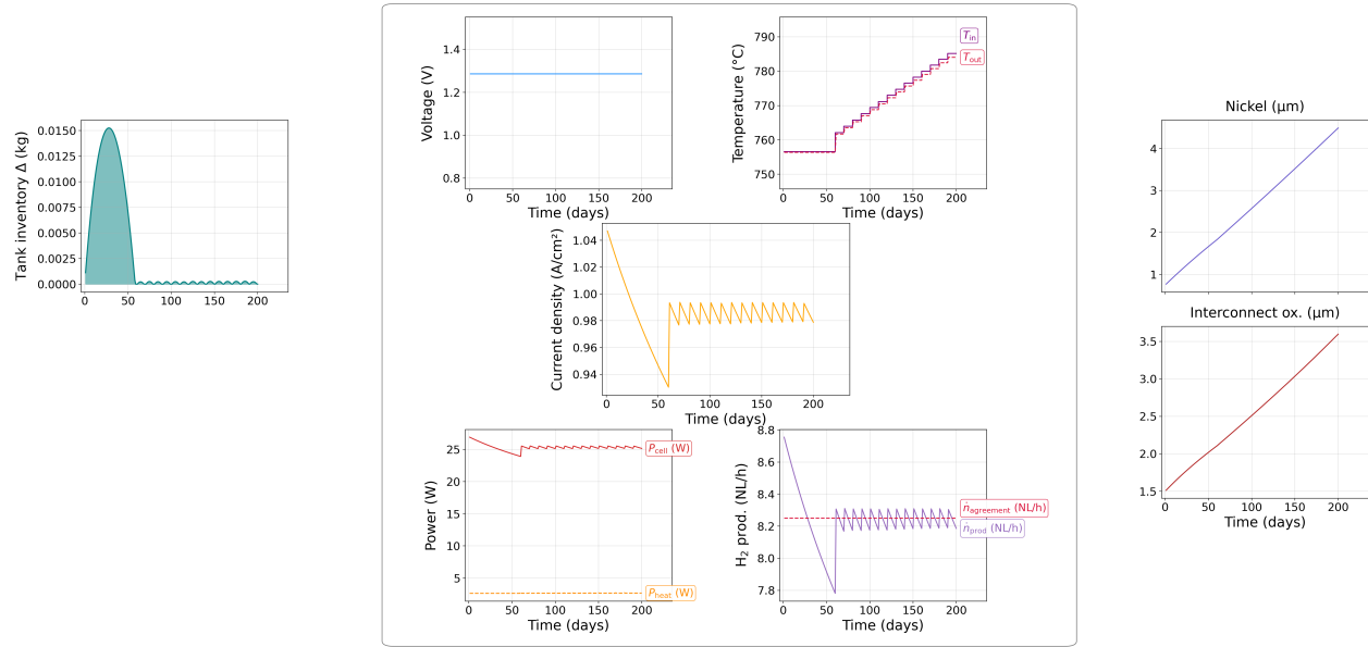
Figure 5.4: Alternative constant-delivery local minimum with the same objective value as Figure 5.3. The optimizer again holds U constant near 1.28 V, but defers galvanostatic scheduling until the tank is exhausted: potentiostatic–isothermal operation continues with fixed T_{\text{in}} \approx 757^\circ\text{C} while degradation lowers \dot{n}_{\text{H}_2, \text{prod}} below \dot{n}_{\text{H}_2, \text{agreement}} and the inventory peak (left panel, \approx 0.015 kg around day 30) is fully consumed by day 60. At that point both temperature and current jump abruptly to galvanostatic tracking of the agreement rate for the remainder of the horizon, with further stepwise increases in T_{\text{in}} compensating degradation. After the switch the tank carries only a small oscillating surplus. Economics are identical to Figure 5.3, but the late, discontinuous mode change makes this trajectory less attractive in practice than maintaining a reserve and reverting to gentler pot-iso operation before the horizon ends.
