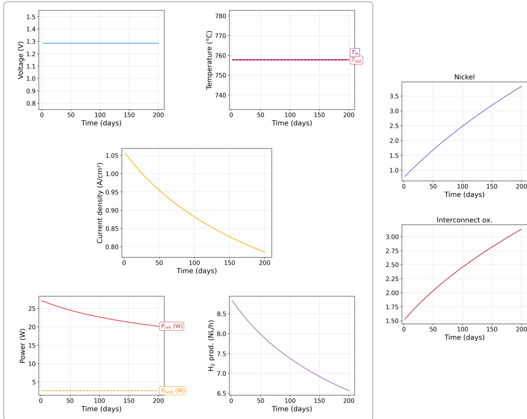
Figure 5.2: Baseline potentiostatic–isothermal optimum with no delivery contract ( N_t = 5 ; settings in Table 5.1). The optimizer returns a single pair of controls, U^* \approx 1.29 V and T_{in}^* \approx 758 °C, broadcast unchanged over the full 200-day horizon (top panels). Operation sits near the thermoneutral point: P_{heat} remains small and T_{out} stays close to T_{in} , so degradation rates are spatially uniform. As nickel migration and interconnect oxidation accumulate (right panels, from 0.75 to \approx 3.7 \mu\text{m} and from 1.5 to \approx 3.1 \mu\text{m} , respectively), potentiostatic control lets current density, cell power, and \dot{n}_{H_2, \text{prod}} decline steadily from about 0.86 A/cm 2 , 22 W, and 7.3 NL/h toward 0.73 A/cm 2 , 18 W, and 6.1 NL/h. Integrated running revenue is 18.99 EUR and terminal salivation 1.45 EUR (net economy 18.53 EUR for the 20 cm 2 cell). The same flat schedule remains optimal when segment-wise control freedom is restored (Section 5.2).
