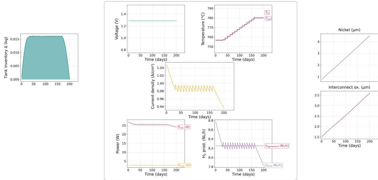
Figure 5.3: Constant-delivery optimum with free voltage and temperature controls ( N_t = 20 ; settings in Table 5.2). One corner case of a continuum of numerically equivalent local minima: after an initial potentiostatic-isothermal phase at the baseline optimum (Section 5.2), inlet temperature is raised in steps so that production tracks the contractual rate \dot{n}_{\text{H}_2, \text{agreement}} = 8.25 \text{ NL/h} (dashed pink line) while U remains fixed near 1.28 V. The tank inventory (left panel) builds to about 0.016 kg by day 40 and is then drawn down only in the final segment, when operation reverts to potentiostatic-isothermal and production falls below the agreement rate. Between these pot-iso bookends, current density and \dot{n}_{\text{H}_2, \text{prod}} oscillate segment-wise around the target—the signature of galvanostatic scheduling achieved through temperature modulation. Nickel migration and interconnect oxidation (right panels) accumulate steadily over the 200-day horizon. Running revenue and terminal salvation match the alternative minimum in Figure 5.4 (15.87 and 1.21 EUR, respectively).
