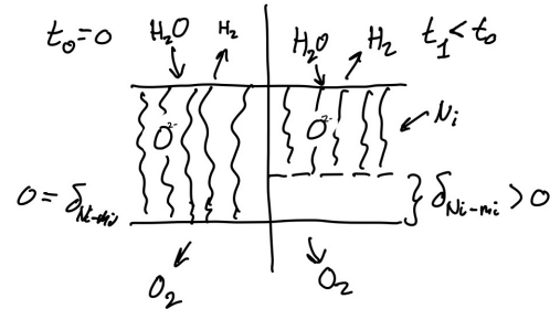
Figure 2.4: For a cell without degradation (left), nickel migration has not occurred and d_{\text{Ni-mi}} = 0 at the layer between the nickel-filled electrode and the electrolyte. Over time the nickel-filled part of the electrode creeps away from the electrolyte (right), giving rise to resistance induced by the raw electrode on the traveling species.
