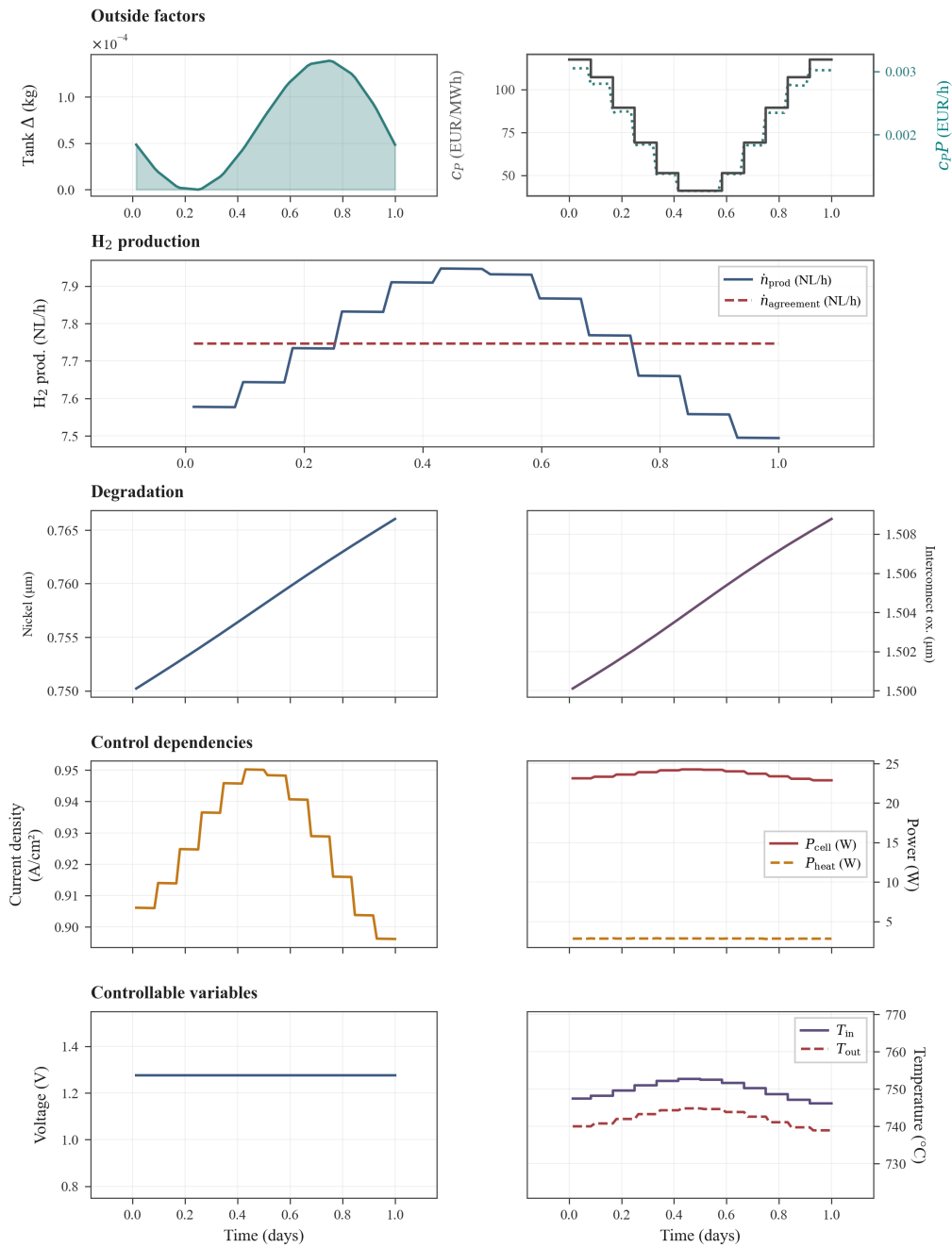
Figure 5.5: 24-hour cyclic optimum under a diurnal power price ( N_t = 12 ; Table 5.4). Fixed U \approx 1.28 V ( w_U = 10 ); T_{\text{in}} is modulated ( w_T = 10^{-3} ) to shift production toward low-price mid-day segments ( c_P and c_P P in Outside factors ). Peak \dot{n}_{\text{H}_2, \text{prod}} \approx 7.95 NL/h versus \approx 7.5 NL/h overnight; the agreement rate is met on average via cyclic tank use ( \kappa_{\text{sell}} = 0 ). Running revenue 0.07 EUR, terminal salvation 1.91 EUR.
