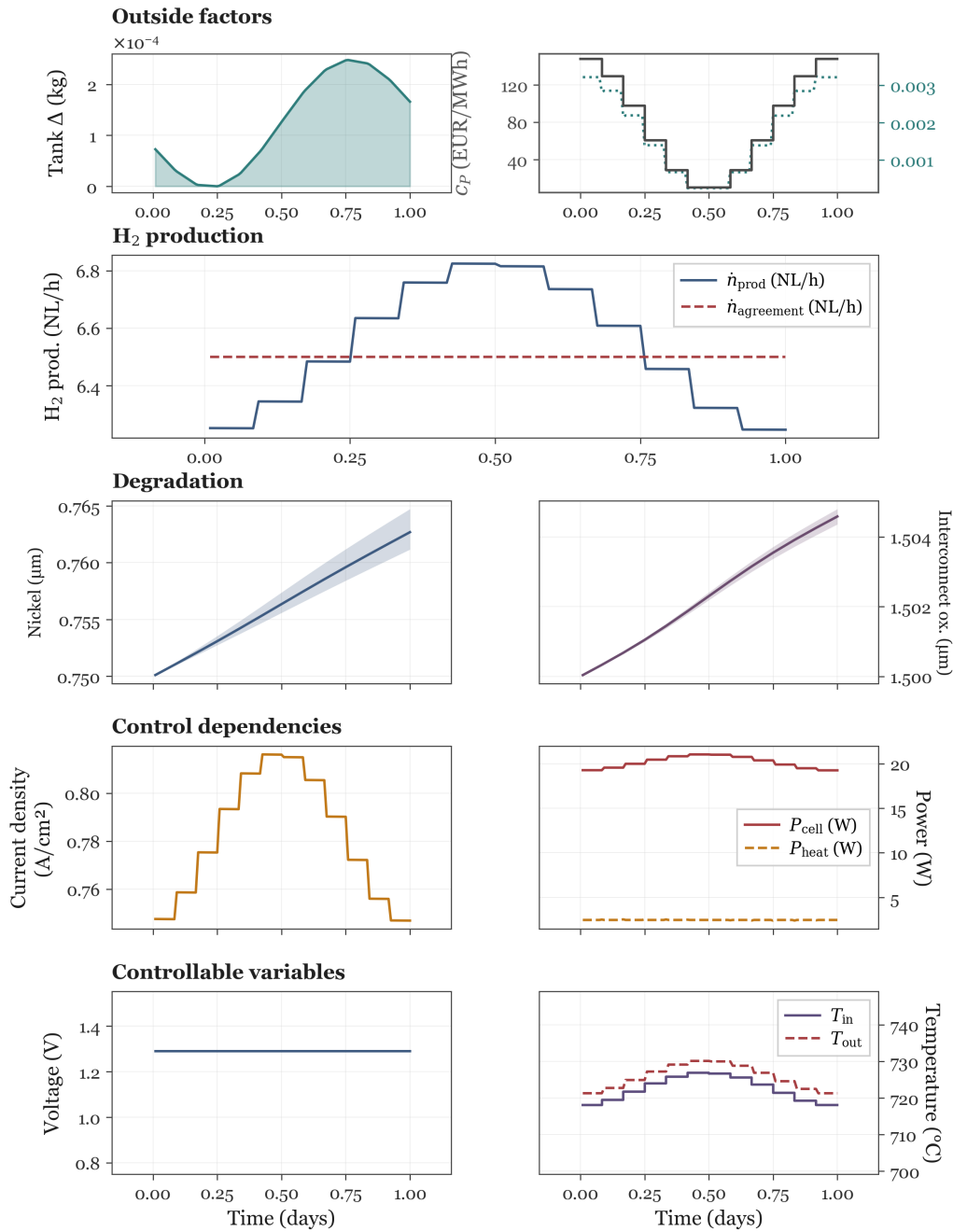
Figure 4.6: 24-hour cyclic optimum under a daily cyclic power price ( N_t = 12 ; table 4.4). Fixed U \approx 1.289 V ( w_U = 0.1 ); T_{in} is modulated ( w_T = 10^{-5} ) to shift production toward low-price midday segments ( c_P and c_{P^*} in Outside factors ). Peak \dot{n}_{H_2,prod} \approx 6.8 NL/h versus \approx 6.2 NL/h overnight; the agreement rate 6.5 NL/h is met on average via cyclic tank use ( \kappa_{sell} = 0 ). Running revenue \Phi \approx 0.062 EUR, terminal salvage \Psi \approx 1.91 EUR.
