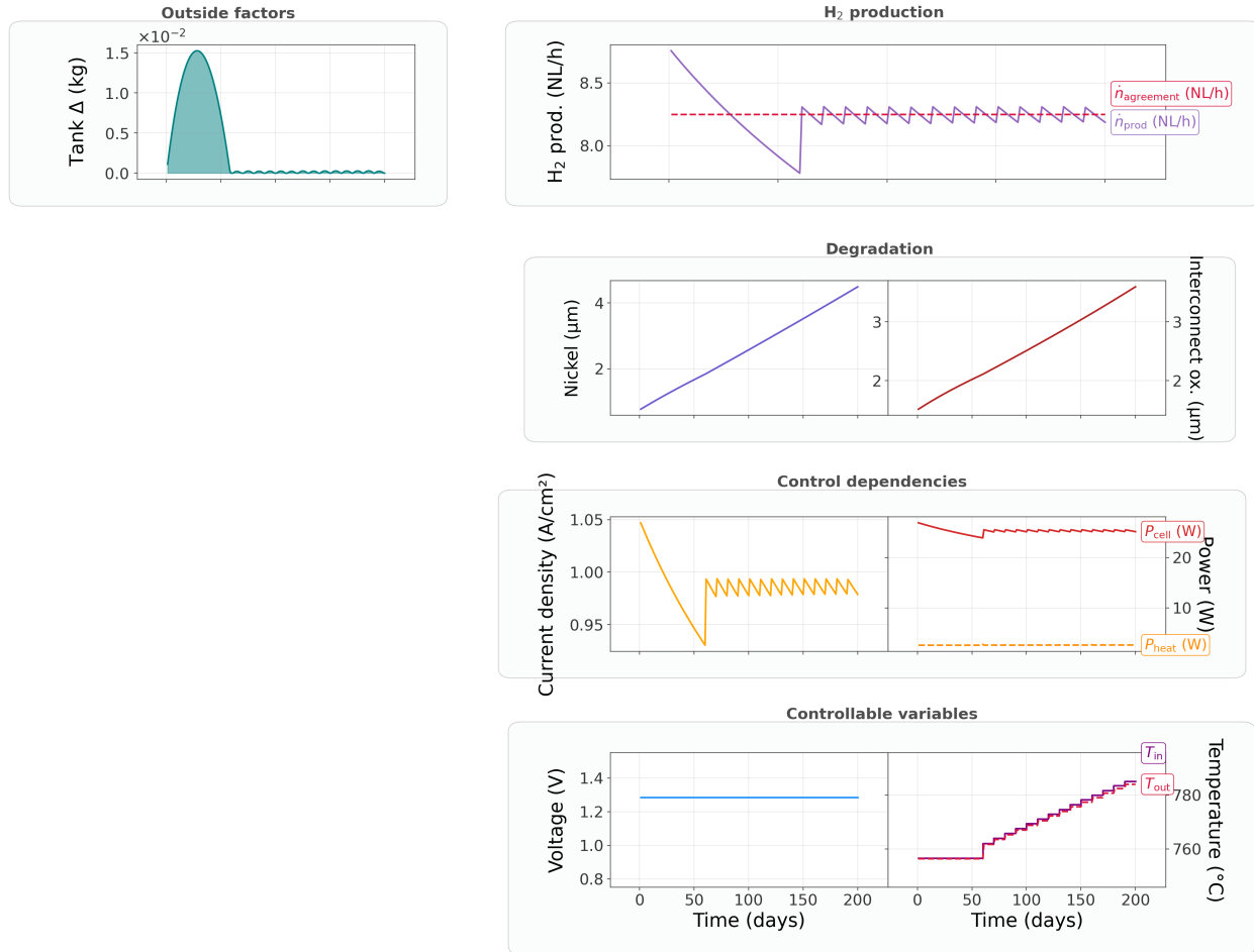
Figure 5.4: Alternative constant-delivery local minimum with the same objective value as Figure 5.3. The optimizer again holds U constant near 1.28 V, but defers galvanostatic scheduling until the tank is exhausted: potentiostatic–isothermal operation continues with fixed T_{\text{in}} \approx 757^\circ\text{C} while degradation lowers \dot{n}_{\text{H}_2, \text{prod}} below \dot{n}_{\text{H}_2, \text{agreement}} and the inventory peak (left panel, \approx 0.015 kg around day 30) is fully consumed by day 60. At that point both temperature and current jump abruptly to galvanostatic tracking of the agreement rate for the remainder of the horizon, with further stepwise increases in T_{\text{in}} compensating degradation. After the switch the tank carries only a small oscillating surplus. Economics are identical to Figure 5.3, but the late, discontinuous mode change makes this trajectory less attractive in practice than maintaining a reserve and reverting to gentler pot-iso operation before the horizon ends.
