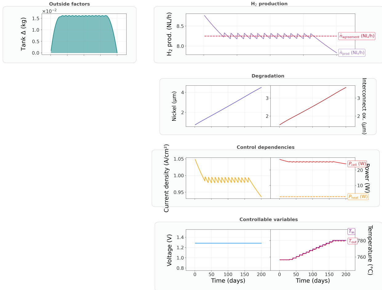
Figure 5.3: Constant-delivery optimum with free voltage and temperature controls ( N_t = 20 ; settings in Table 5.3). One corner case of a continuum of numerically equivalent local minima: after an initial potentiostatic-isothermal phase at the baseline optimum (Section 5.2), inlet temperature is raised in steps so that production tracks the contractual rate \dot{n}_{\text{H}_2, \text{agreement}} = 8.25 \text{ NL/h} (dashed pink line) while U remains fixed near 1.28 V. The tank inventory (left panel) builds to about 0.016 kg by day 40 and is then drawn down only in the final segment, when operation reverts to potentiostatic-isothermal and production falls below the agreement rate. Between these pot-iso bookends, current density and \dot{n}_{\text{H}_2, \text{prod}} oscillate segment-wise around the target—the signature of galvanostatic scheduling achieved through temperature modulation. Nickel migration and interconnect oxidation (right panels) accumulate steadily over the 200-day horizon. Running revenue and terminal salvation match the alternative minimum in Figure 5.4 (15.87 and 1.21 EUR, respectively).
