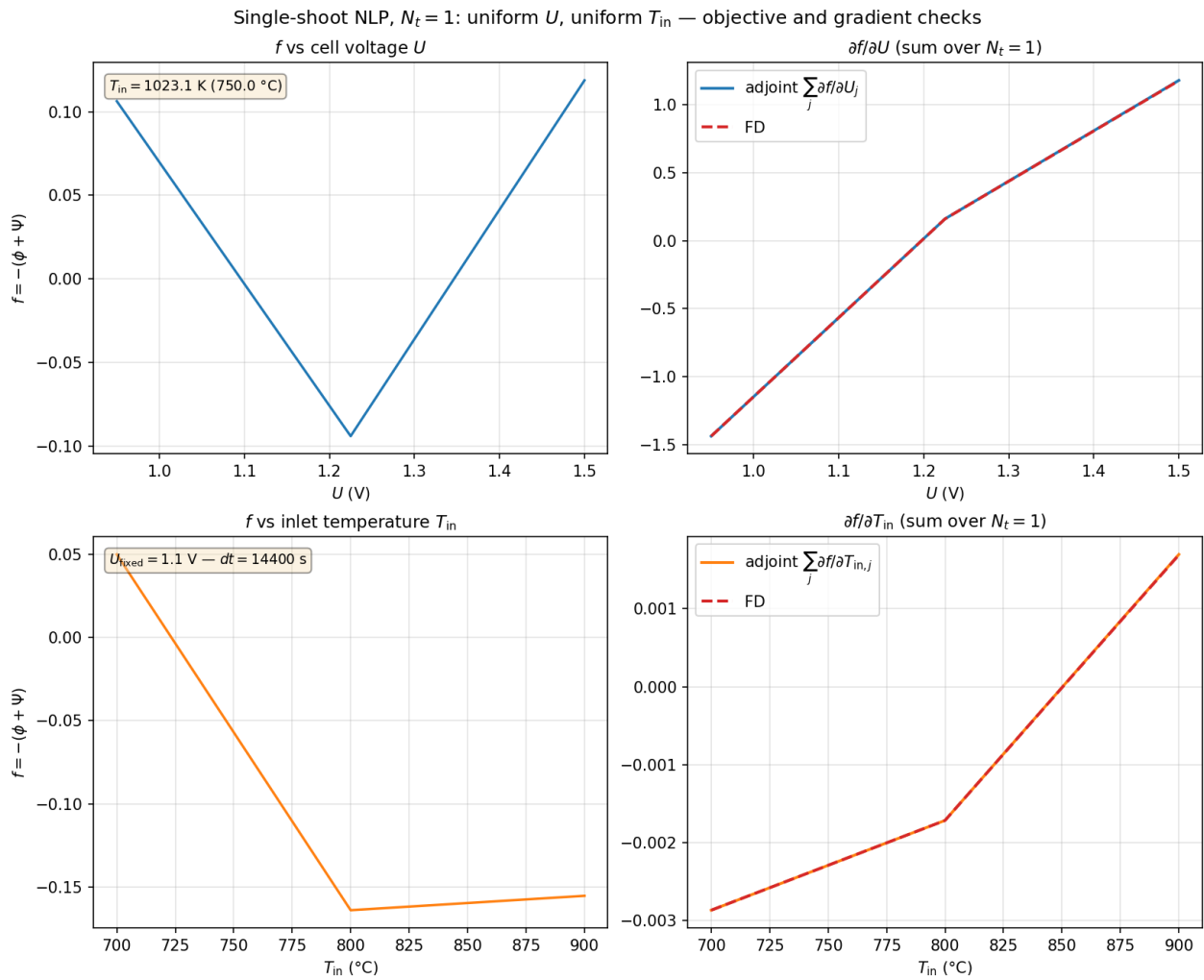
Figure A7.1: Single-shooting NLP gradient check at N_t = 1 : objective f = -(\phi + \psi) and its derivatives w.r.t. uniform cell voltage U (top) and inlet temperature T_{in} (bottom). Solid lines: adjoint; dashed: central FD with all segment controls perturbed together.
