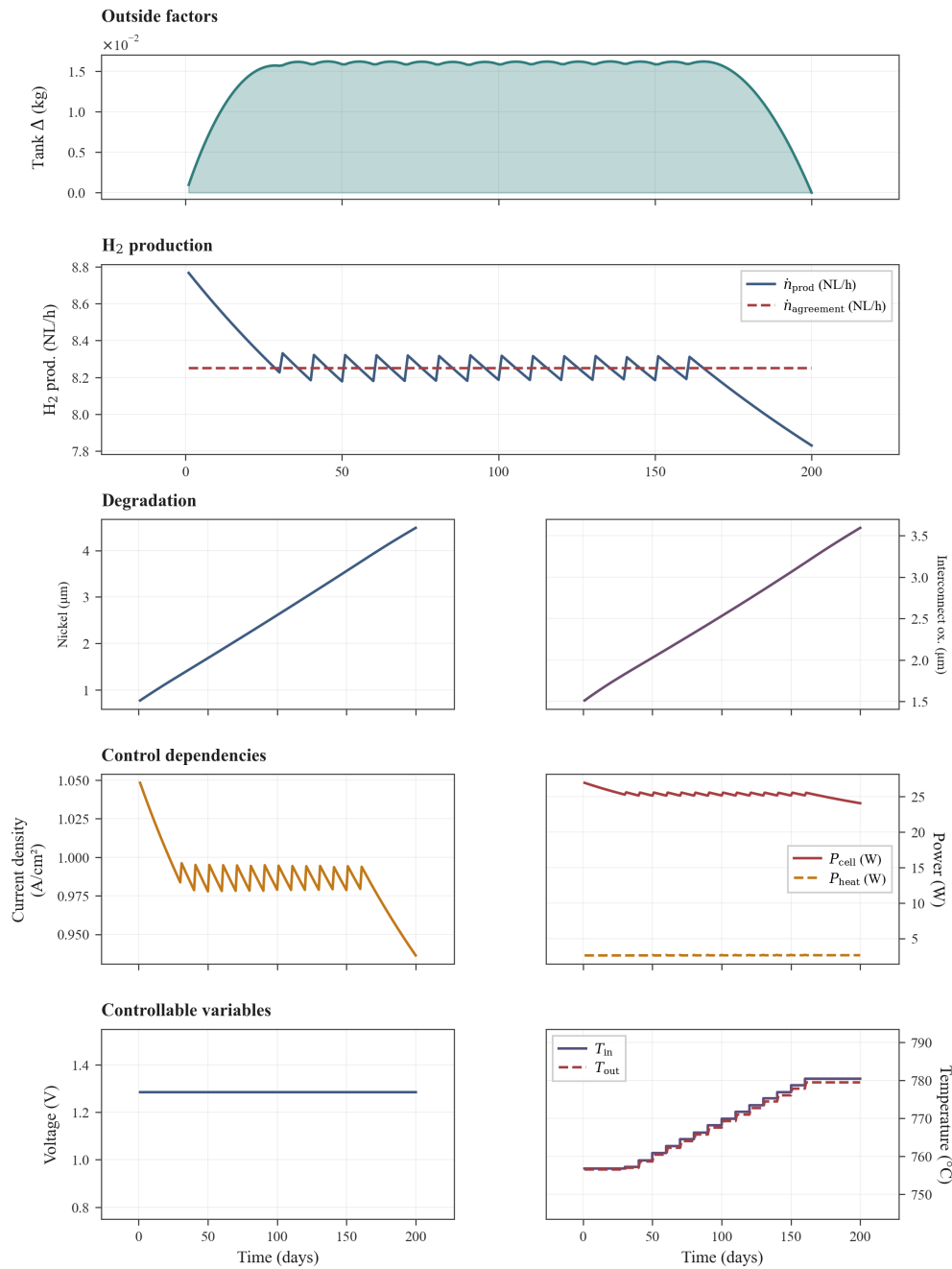
Figure 5.3: Constant-delivery optimum with free voltage and temperature ( N_t = 20 ; Table 5.3). One corner case among degenerate minima (Figure 5.4): pot-iso bookends at U \approx 1.28 V bracket galvanostatic tracking of \dot{n}_{\text{H}_2, \text{agreement}} = 8.25 NL/h via stepped T_{\text{in}} . Tank inventory peaks at \approx 0.016 kg (day 40) and is drawn down only in the closing pot-iso phase. Running revenue 15.87 EUR, terminal salvation 1.21 EUR.
