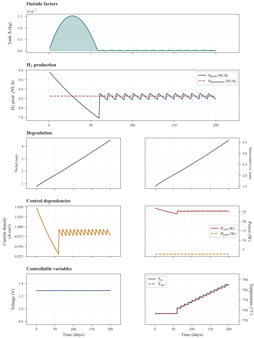
Figure 5.4: Alternative constant-delivery local minimum, same objective as Figure 5.3. Galvanostatic scheduling is deferred until the tank is exhausted (peak \approx 0.015 kg around day 30, empty by day 60); U stays near 1.28 V with T_{\text{in}} \approx 757^{\circ}\text{C} until an abrupt switch to agreement-rate tracking. Economics match Figure 5.3, but the late discontinuous mode change is less attractive operationally.
