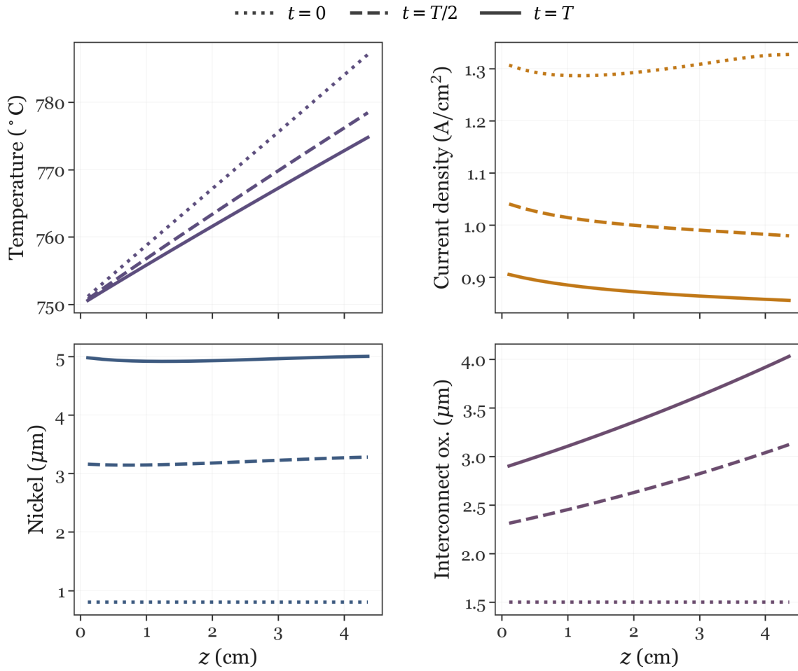
Figure 4.3: Spatial channel profiles at t = 0 , t = t_{\text{horizon}}/2 , and t = t_{\text{horizon}} for the baseline pot-iso optimum (fine forward replay). Temperature rises along z under exothermal operation; nickel migration approaches the 5 \mu\text{m} critical degradation limit almost uniformly at t = t_{\text{horizon}} , while interconnect oxidation stays below its limit with stronger outlet weighting.
