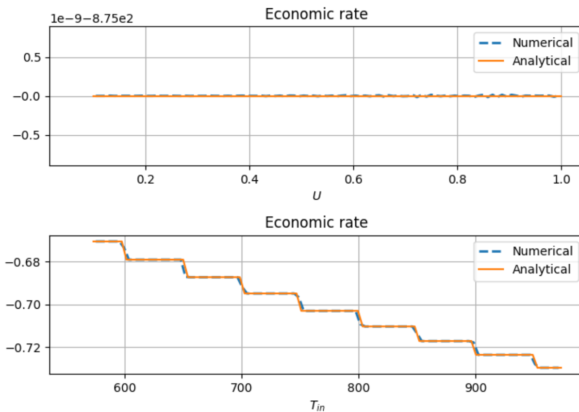
Figure A7.4: Gradient verification output: economic_rate_dp.png.
