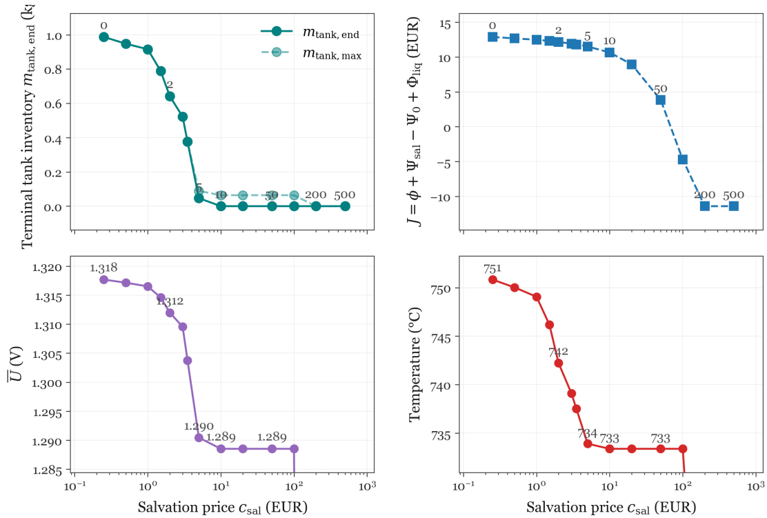
Figure 5.9: Salvation price c_{\text{sal}} sensitivity at fixed \kappa_{\text{sell}} = 40.74\% and \dot{n}_{\text{H}_2, \text{agreement}} = 6.5 \text{ NL/h} (pot-iso controls). Top panels: Terminal and peak tank inventory and net objective J ; bottom panels: Mean voltage and inlet temperature. At the baseline price (2 EUR, starred) the optimizer hoards \approx 0.64 \text{ kg} by running the cell hard. As c_{\text{sal}} rises, inventory falls and J decreases; above \approx 10 \text{ EUR} the optimum reverts to gentle pot-iso operation with negligible terminal inventory.
