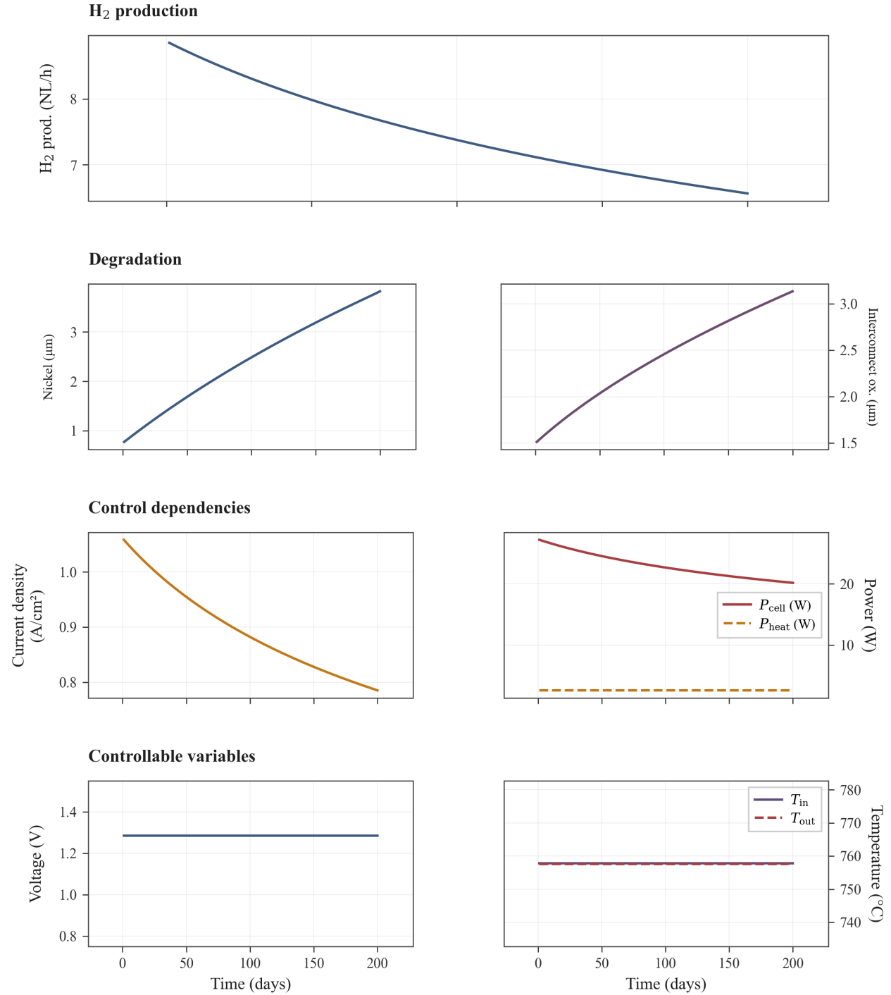
Figure 5.2: Baseline potentiostatic–isothermal optimum with no delivery contract ( N_t = 5 ; settings in Table 5.1). Rows (top to bottom): H 2 production , Degradation , Control dependencies , and Controllable variables . The optimizer returns a single pair of controls, U^* \approx 1.29 V and T_{in}^* \approx 758 °C, held constant over the full 200-day horizon. Operation sits near the thermoneutral point: P_{heat} remains small and T_{out} stays close to T_{in} ( Control dependencies and Controllable variables ), so degradation rates stay spatially uniform. Nickel migration and interconnect oxidation ( Degradation ) grow from 0.75 to \approx 3.7 \mu\text{m} and from 1.5 to \approx 3.1 \mu\text{m} , respectively; under potentiostatic control, current density, cell power, and \dot{n}_{H_2,prod} decline steadily from about 0.86 A/cm 2 , 22 W, and 7.3 NL/h toward 0.73 A/cm 2 , 18 W, and 6.1 NL/h. Integrated running revenue is 18.99 EUR and terminal
