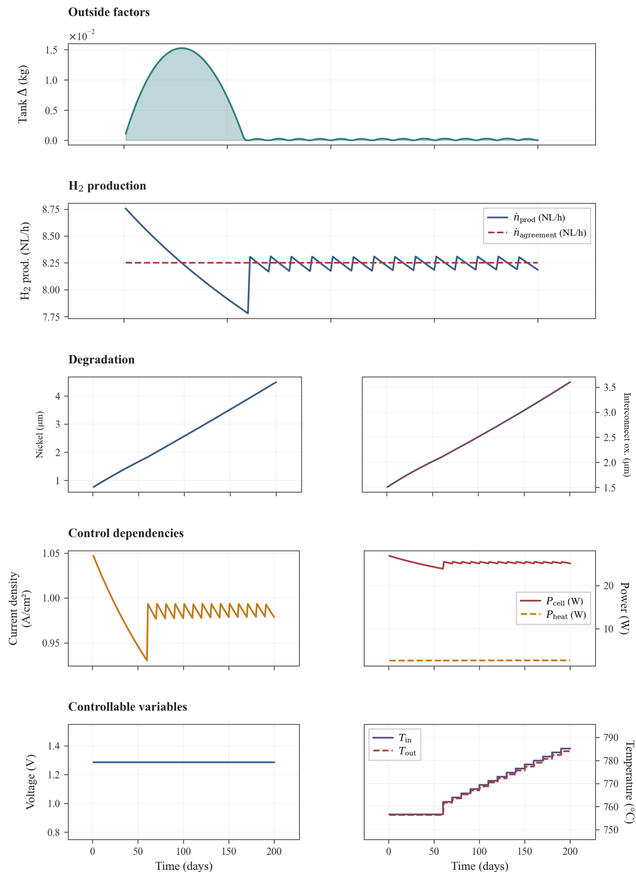
Figure 5.4: Alternative constant-delivery local minimum with the same objective value as Figure 5.3. Rows (top to bottom): Outside factors , H 2 production , Degradation , Control dependencies , and Controllable variables . The optimizer again holds
