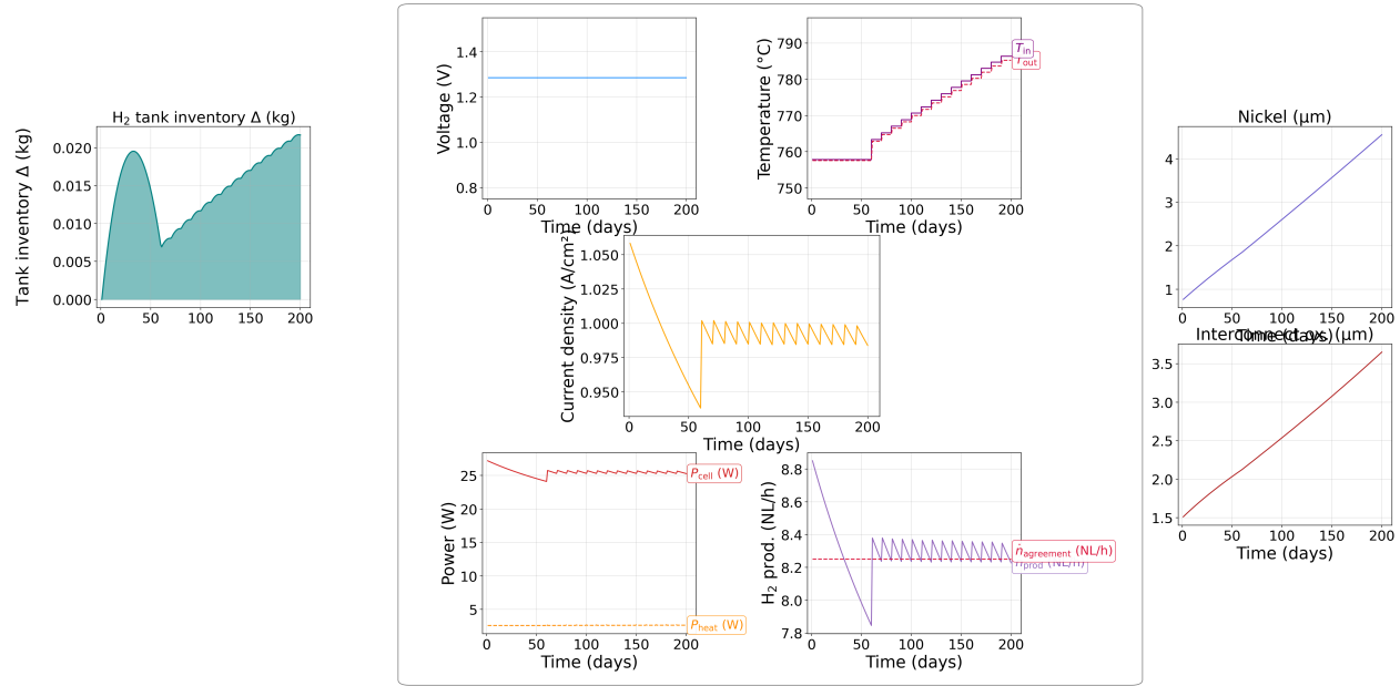
Figure 6.4: Alternative constant-delivery local minimum with the same objective value as Figure 6.3. The optimizer again holds U constant near 1.28 V, but defers galvanostatic scheduling until the tank is exhausted: potentiostatic–isothermal operation continues with fixed T_{\text{in}} \approx 757^\circ\text{C} while degradation lowers \dot{n}_{\text{H}_2, \text{prod}} below \dot{n}_{\text{H}_2, \text{agreement}} and the inventory peak (left panel, \approx 0.015 kg around day 30) is fully consumed by day 60. At that point both temperature and current jump abruptly to galvanostatic tracking of the agreement rate for the remainder of the horizon, with further stepwise increases in T_{\text{in}} compensating degradation. After the switch the tank carries only a small oscillating surplus. Economics are identical to Figure 6.3, but the late, discontinuous mode change makes this trajectory less attractive in practice than maintaining a reserve and reverting to gentler pot-iso operation before the horizon ends.
