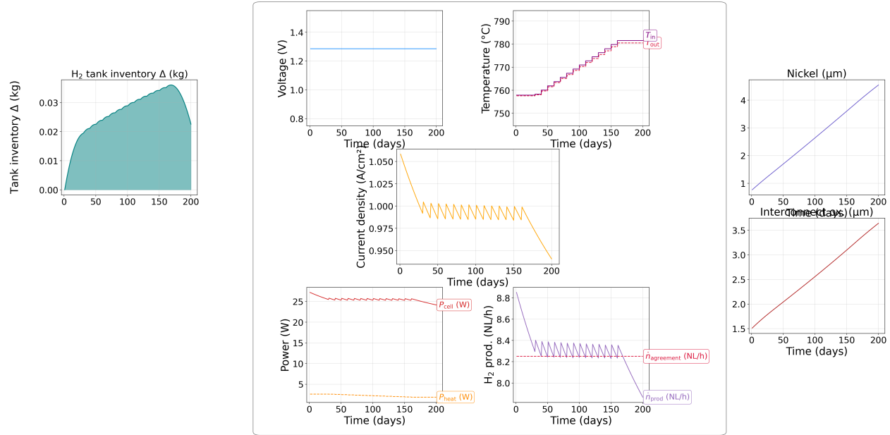
Figure 6.3: Constant-delivery optimum with free voltage and temperature controls ( N_t = 20 ; settings in Table 6.2). One corner case of a continuum of numerically equivalent local minima: after an initial potentiostatic-isothermal phase at the baseline optimum (Section 6.2), inlet temperature is raised in steps so that production tracks the contractual rate \dot{n}_{\text{H}_2, \text{agreement}} = 8.25 \text{ NL/h} (dashed pink line) while U remains fixed near 1.28 V. The tank inventory (left panel) builds to about 0.016 kg by day 40 and is then drawn down only in the final segment, when operation reverts to potentiostatic-isothermal and production falls below the agreement rate. Between these pot-iso bookends, current density and \dot{n}_{\text{H}_2, \text{prod}} oscillate segment-wise around the target—the signature of galvanostatic scheduling achieved through temperature modulation. Nickel migration and interconnect oxidation (right panels) accumulate steadily over the 200-day horizon. Running revenue and terminal salvation match the alternative minimum in Figure 6.4 (15.87 and 1.21 EUR, respectively).
