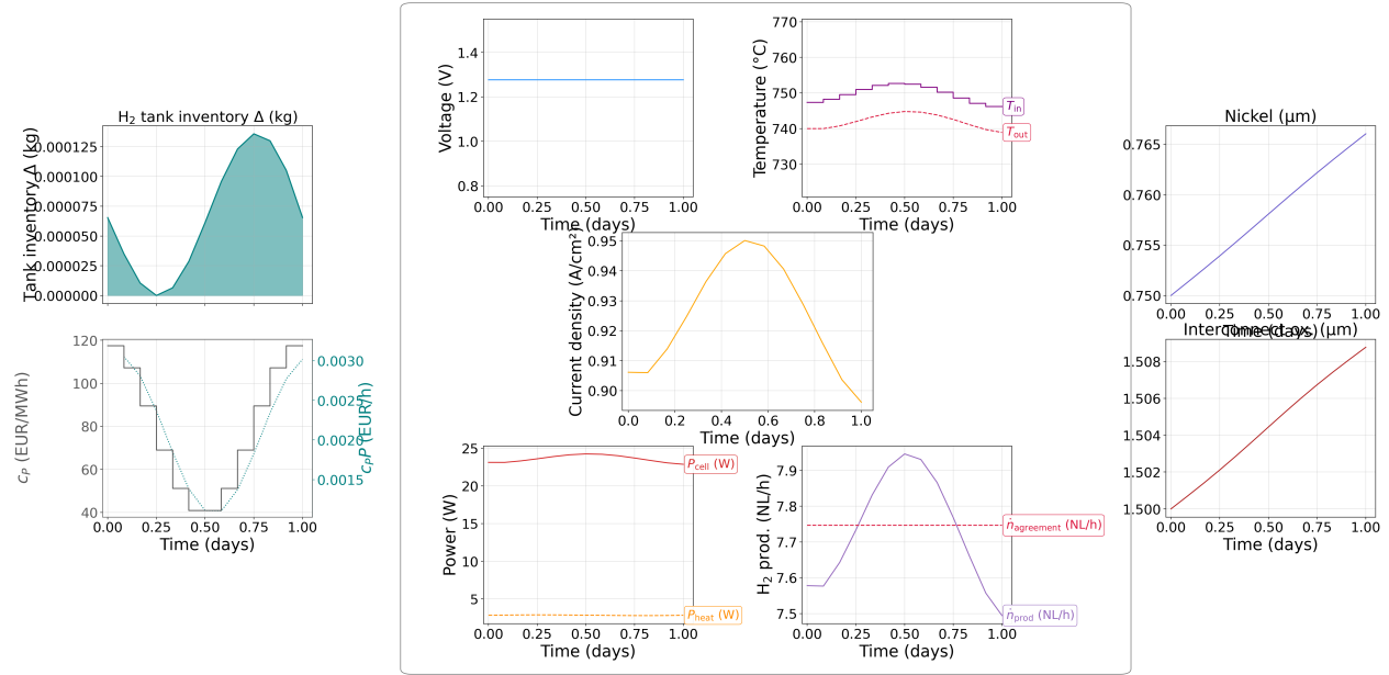
Figure 6.5: 24-hour cyclic optimum under a diurnal power price ( N_t = 12 ; settings in Table 6.3). Voltage is held potentiostatic near 1.28 V ( w_U = 10 ), and inlet temperature is the primary free control ( w_T = 10^{-3} ). The piecewise-constant electricity price c_{P,k} (bottom-left panel) follows a single cosine cycle with its minimum at midday and maximum at midnight; the corresponding hydrogen revenue rate c_{H_2}P mirrors this pattern. In response, T_{in} is raised in steps through the cheap midday segments, lifting current density and \dot{n}_{H_2,prod} to a peak of about 7.95 NL/h while production is throttled to \approx 7.5 NL/h overnight. The contractual rate \dot{n}_{H_2,agreement} (dashed red line) is met on average via the tank: inventory (top-left panel) is drawn down in the morning, rebuilt during low-price production, and returned to its initial level at t = 24 h ( \kappa_{sell} = 0 ). Degradation over one day is negligible (right panels). Integrated running revenue is 0.07 EUR and terminal salvation 1.91 EUR.
