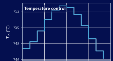
24-hour optimal schedule: load shifting with buffer storage Potentialostatic SOEC · diurnal power price · contractual H 2 delivery
