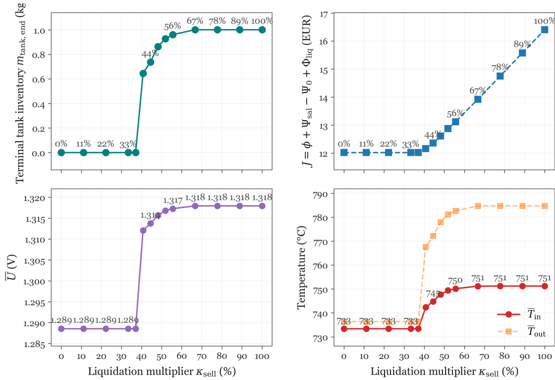
Figure 4.7: Terminal liquidation credit \kappa_{\text{sell}} sensitivity for the constant-delivery tank scenario ( \dot{n}_{\text{H}_2, \text{agreement}} = 6.5 \text{ NL/h} , pot-iso controls, no tank cap). Top panels: Terminal tank inventory and net objective J = \phi + \Psi_{\text{sal}} - \Psi_0 + \Phi_{\text{liq}} ; bottom panels: Mean voltage and inlet/outlet temperature. For \kappa_{\text{sell}} \lesssim 37\% the optimizer leaves the tank empty and holds moderate U and T_{\text{in}} . Above \approx 40\% it hoards surplus hydrogen and drives the cell toward the nickel critical degradation limit.
