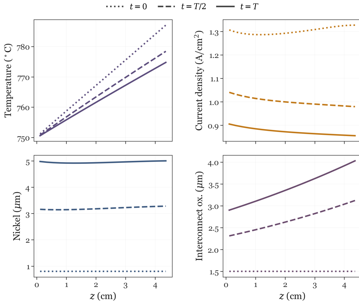
Figure 4.3: Spatial channel profiles at t = 0 , t = T/2 , and t = T for the baseline pot-iso optimum (fine forward replay). Temperature rises along z under exothermal operation; nickel migration approaches the 5 \mu\text{m} break limit almost uniformly at t = T , while interconnect oxidation stays below its cap with stronger outlet weighting.
