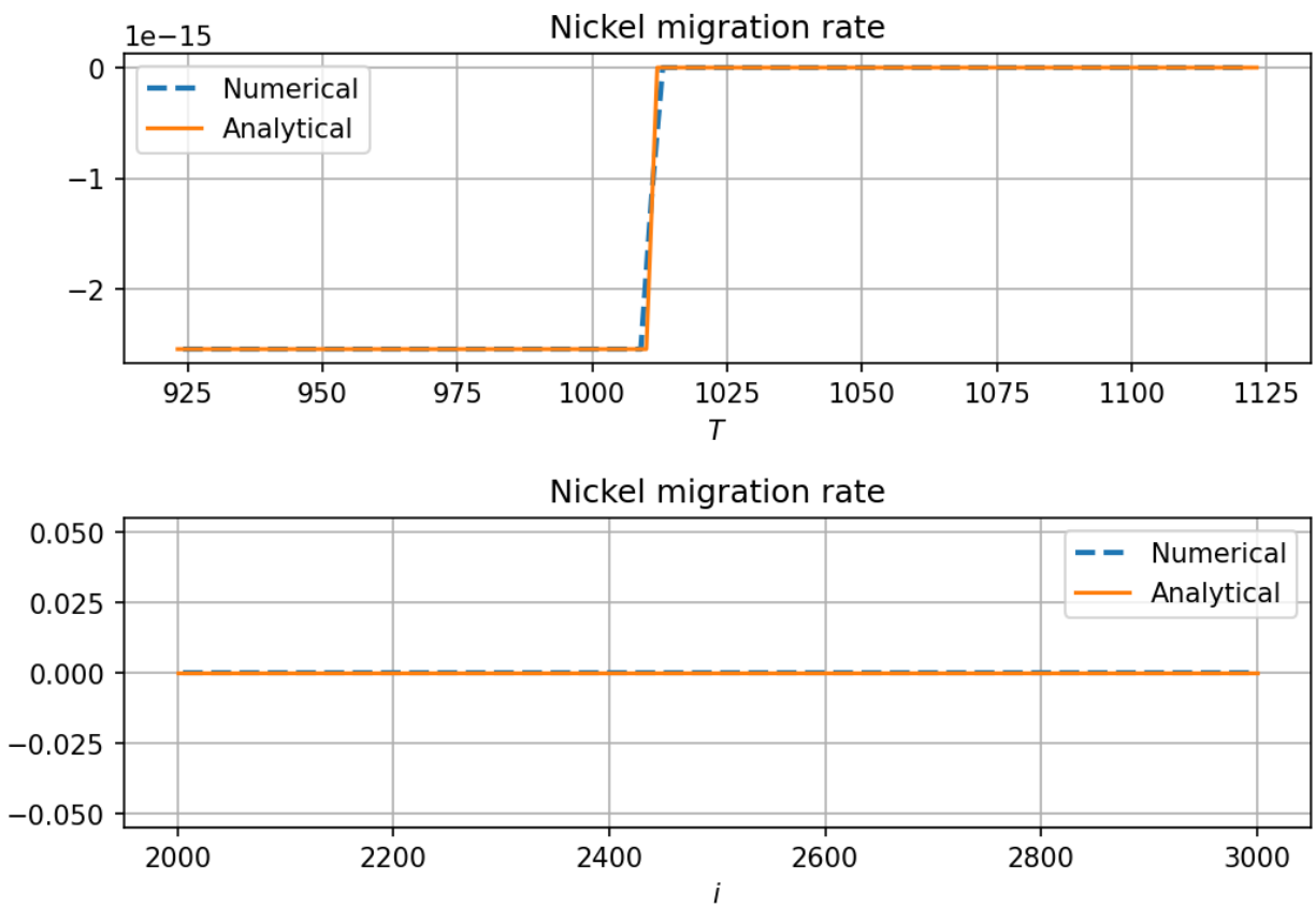
Figure A6.29: Gradient verification output: nickel_migration_rate.png.
