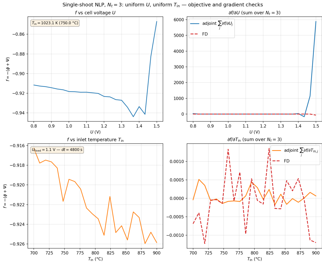
Figure A6.36: Gradient verification output: nlp_gradients_NT3.png.
