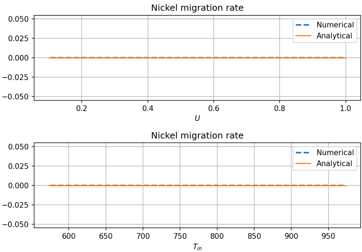
Figure A6.30: Gradient verification output: nickel_migration_rate_dp.png.
