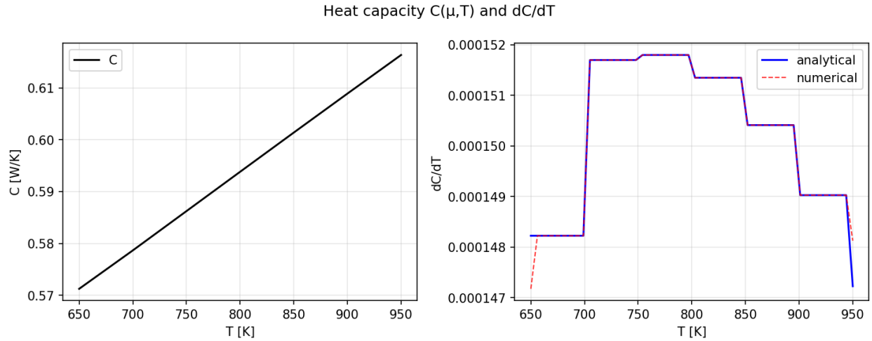
Figure A6.16: Gradient verification output: gradient_test_heat_capacity.png.
