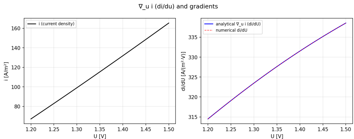
Figure A6.18: Gradient verification output: gradient_test_nabla_u.png.
