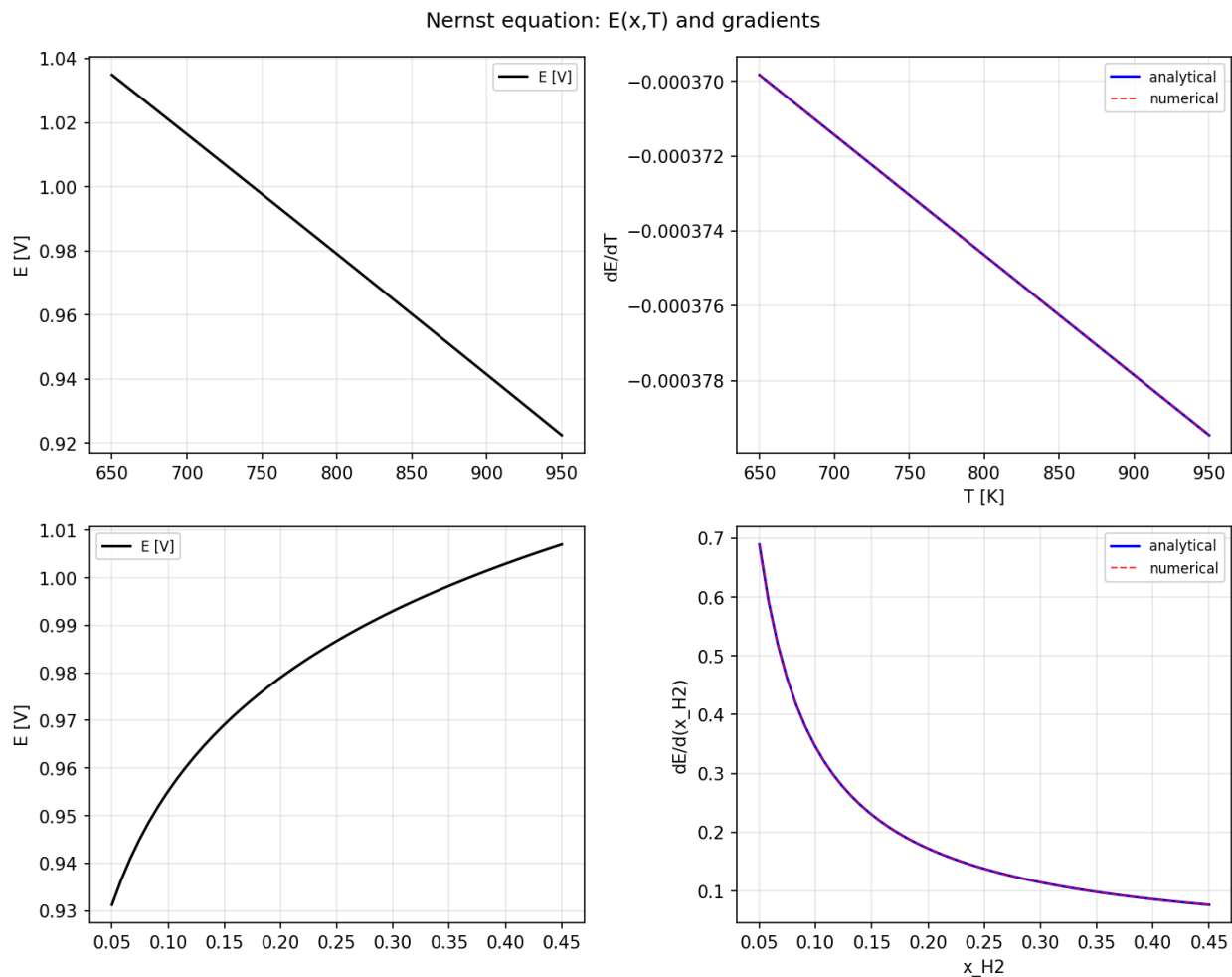
Figure A6.19: Gradient verification output: gradient_test_nernst.png.
