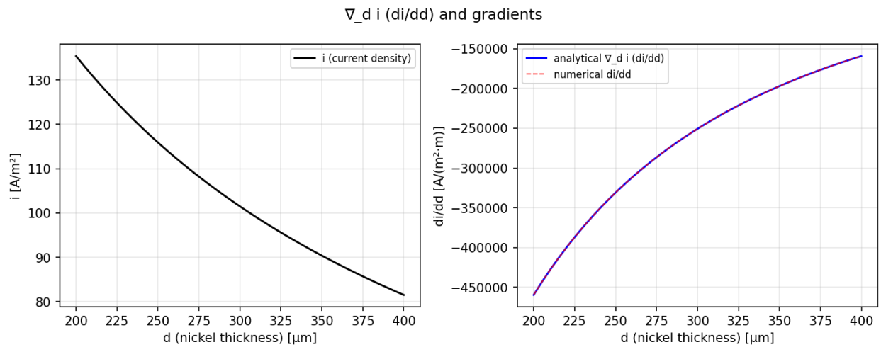
Figure A6.17: Gradient verification output: gradient_test_nabla_d.png.
