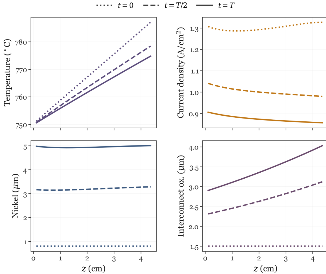
Figure 5.3: Spatial channel profiles at t=0 , t=T/2 , and t=T for the baseline pot-iso optimum (fine forward replay). Temperature rises along z under exothermal operation; nickel migration approaches the 5 \mu\text{m} break limit almost uniformly at t=T , while interconnect oxidation stays below its cap with stronger outlet weighting.
