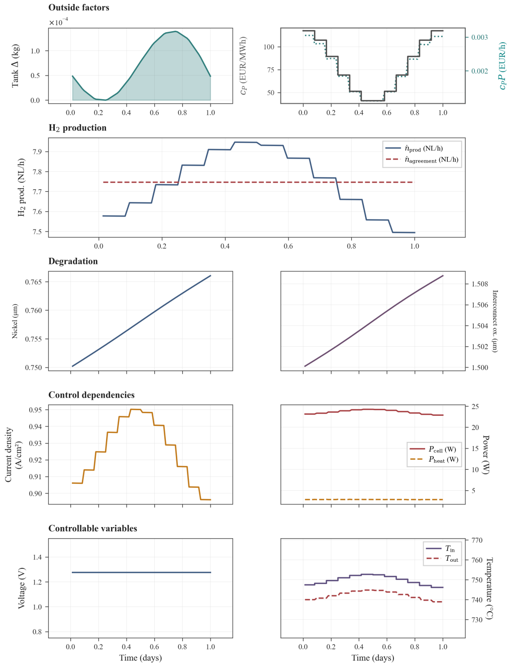
Figure 5.7: 24-hour cyclic optimum under a diurnal power price ( N_t = 12 ; Table 5.5). Figure pending re-run with a = 0.9 , periodic continuity wrap, and updated optimizer settings; values below are from an earlier a = 0.5 run. Fixed U \approx 1.28 V ( w_U = 10 ); T_{\text{in}} is modulated ( w_T = 10^{-3} ) to shift production toward low-price midday segments ( c_P and c_P P in Outside factors ). Peak \dot{n}_{\text{H}_2, \text{prod}} \approx 7.95 NL/h versus \approx 7.5 NL/h overnight; the agreement rate is met on average via cyclic tank use ( \kappa_{\text{sell}} = 0 ). Running revenue 0.07 EUR, terminal salvation 1.91 EUR.
