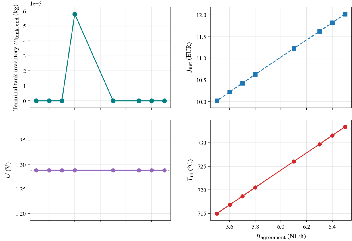
Figure 5.6: Agreement-rate sensitivity at \kappa_{\text{sell}} = 0 and pot-iso controls ( N_t = 20 ). U is fixed to the 6.5 NL/h optimum ( \approx 1.289 V); T_{\text{in}} is reduced per case so that m_{\text{tank, end}} = 0 . J_{\text{net}} = \phi + \Psi_{\text{sal}} - \Psi_0 .
