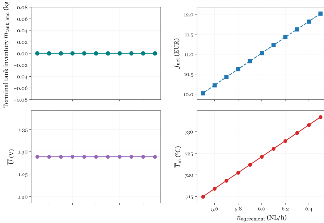
Figure 4.10: Contractual delivery rate sensitivity at \kappa_{\text{sell}} = 0 and pot-iso controls ( N_t = 20 ). U is fixed to the 6.5 NL/h optimum ( \approx 1.289 V); T_{\text{in}} is reduced for lower agreement rates so that m_{\text{tank, end}} = 0 . Top panels: Terminal tank inventory and net objective J_{\text{net}} ; bottom panels: Mean voltage and inlet temperature. J_{\text{net}} rises almost linearly from \approx 10.0 to \approx 12.0 EUR as \dot{n}_{\text{H}_2, \text{agreement}} increases from 5.5 to 6.5 NL/h. Voltage stays flat while \bar{T}_{\text{in}} falls from \approx 734 to \approx 715 °C.
