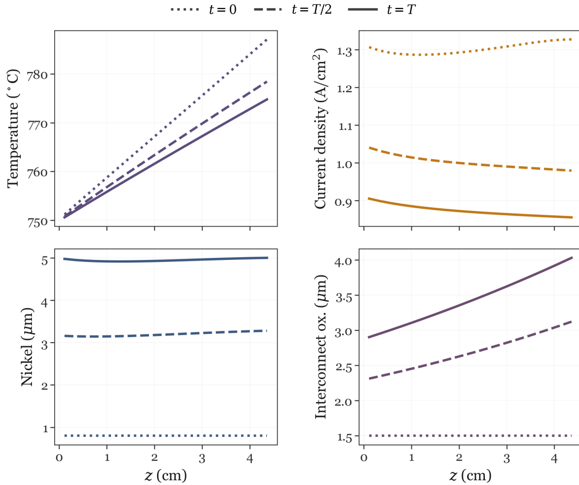
Figure 4.3: Spatial channel profiles at t = 0 , t = T/2 , and t = T for the baseline pot-iso optimum (fine forward replay). Temperature rises along z under exothermal operation; nickel migration approaches the 5 \mu\text{m} break limit almost uniformly at t = T , while interconnect oxidation stays below its cap with stronger outlet weighting.
