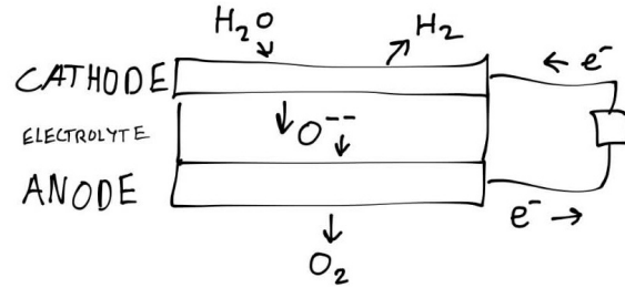
Figure 2.2: A sketch of a unit cell: The basic principles of an SOEC cell are illustrated. The cathode pulls apart the hydrogen and oxygen in the water. The oxygen is transferred through the electrolyte, then formed to dioxygen in the anode, all due to an applied current.
