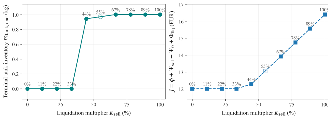
Figure 6.1: Sensitivity on the resale price from the leftover tank content at the end time. Here we see the tank content plotted at the left plot and the net revenue plotted on the right plot. The faded point at 55% is here because the optimizer failed to find an optimum for this value. Here it is clear to see that we find a breaking point for which the hydrogen price hits a low enough value that it is not worth producing. For a very small window it makes sense to produce less than the optimum to save the cell.
