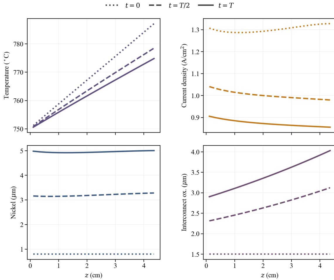
Figure 5.3: Spatial channel profiles at t = 0 , t = T/2 , and t = T for the baseline pot-iso optimum (fine forward replay). Temperature rises along z under exothermal operation; nickel migration approaches the 5 \mu\text{m} break limit almost uniformly at t = T , while interconnect oxidation stays below its cap with stronger outlet weighting.
