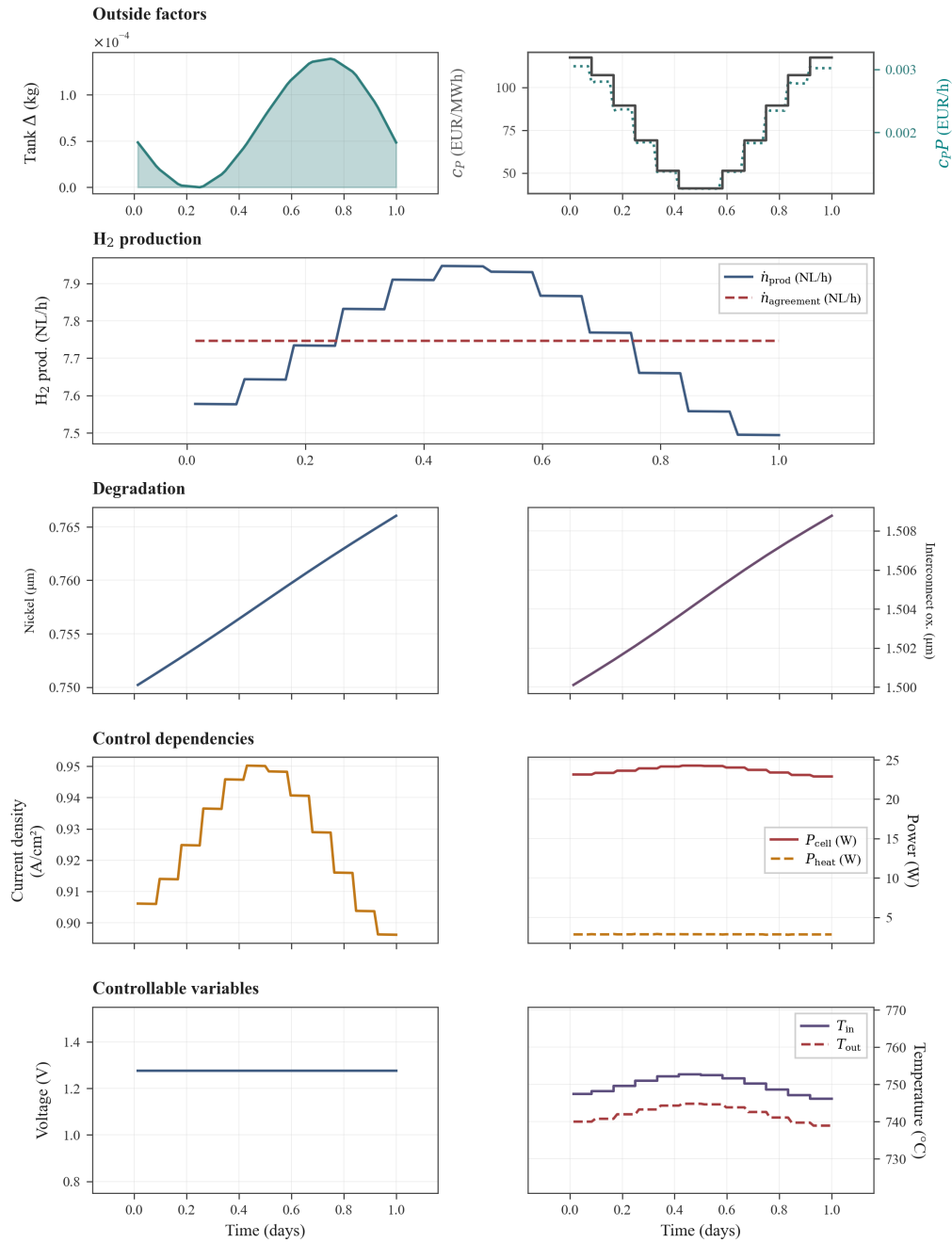
Figure 5.5: 24-hour cyclic optimum under a diurnal power price ( N_t = 12 ; Table 5.5). Figure pending re-run with a = 0.9 , periodic continuity wrap, and updated optimizer settings; values below are from an earlier a = 0.5 run. Fixed U \approx 1.28 V ( w_U = 10 ); T_{\text{in}} is modulated ( w_T = 10^{-3} ) to shift production toward low-price midday segments ( c_P and c_P P in Outside factors ). Peak \dot{n}_{\text{H}_2, \text{prod}} \approx 7.95 NL/h versus \approx 7.5 NL/h overnight; the agreement rate is met on average via cyclic tank use ( \kappa_{\text{sell}} = 0 ). Running revenue 0.07 EUR, terminal salvation 1.91 EUR.
