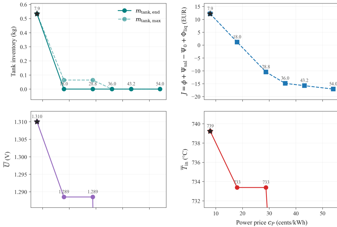
Figure 5.7: Power price c_P sensitivity at fixed \kappa_{\text{sell}} = 40.74\% and \dot{n}_{\text{H}_2, \text{agreement}} = 6.5 \text{ NL/h} (pot-iso controls). Top panels: terminal and peak tank inventory and net objective J ; bottom panels: mean voltage and inlet temperature. At the baseline price ( \approx 7.9 cent/kWh, starred) the optimizer hoards \approx 0.53 kg by running the cell hard. As c_P rises, inventory falls and J decreases while production is kept alive down to \approx 29 cent/kWh. Above \approx 36 cent/kWh electrolysis shuts down and contract hydrogen is purchased at spot.
