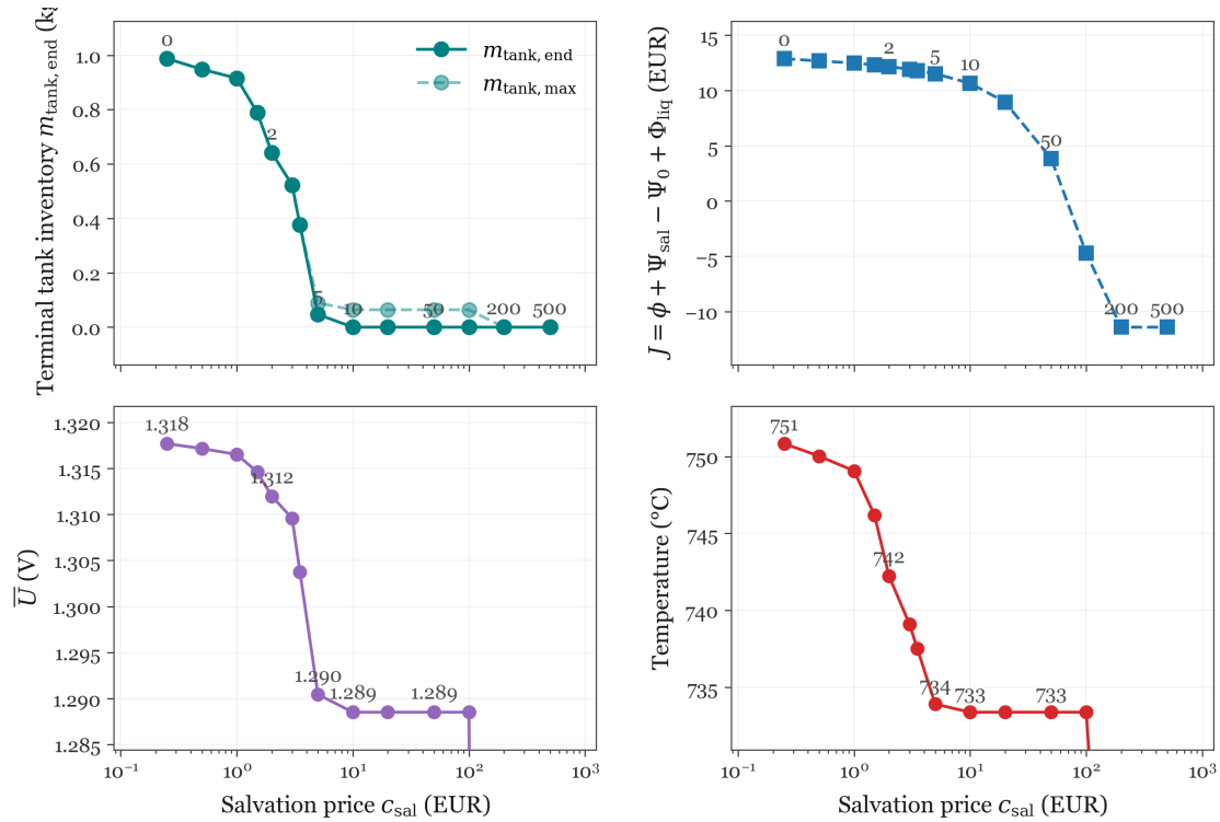
Figure 5.9: salvage price c_{sal} sensitivity at fixed \kappa_{sell} = 40.74\% and \dot{n}_{H_2,agreement} = 6.5 NL/h (pot-iso controls). Top panels: Terminal and peak tank inventory and net objective J ; bottom panels: Mean voltage and inlet temperature. At the baseline price (2 EUR, starred) the optimizer hoards \approx 0.64 kg by running the cell hard. As c_{sal} rises, inventory falls and J decreases; above \approx 10 EUR the optimum reverts to gentle pot-iso operation with negligible terminal inventory.
