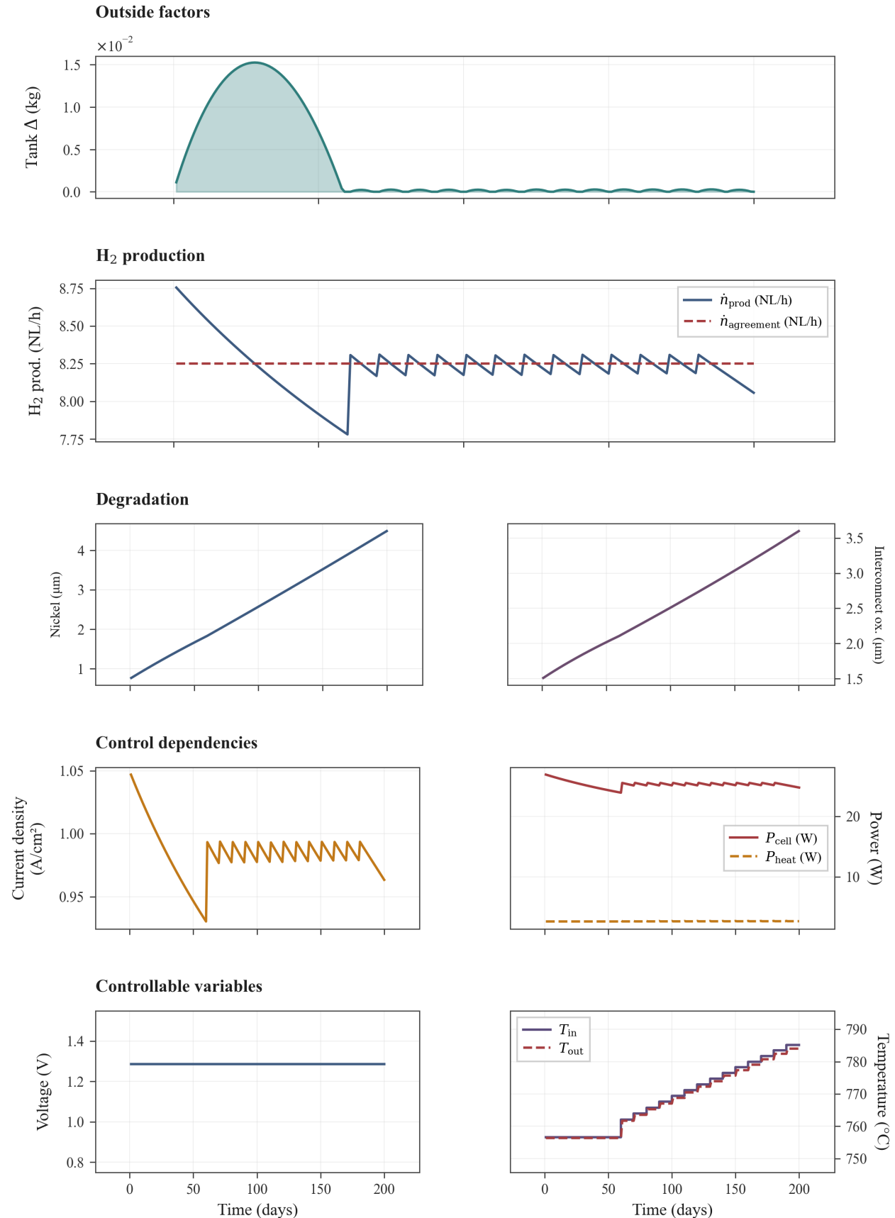
Figure 5.4: Alternative constant-delivery local minimum with the same objective value as Figure 5.3. The optimizer again holds U constant near 1.28 V, but defers galvanostatic scheduling until the tank is exhausted: potentiostatic–isothermal operation continues with fixed T_{\text{in}} \approx 757^{\circ}\text{C} while degradation lowers \dot{n}_{\text{H}_2, \text{prod}} below \dot{n}_{\text{H}_2, \text{agreement}} and the inventory peak (left panel, \approx 0.015 kg around day 30) is fully consumed by day 60. At that point both temperature and current are allowed to vary to enable constant tracking of the agreement rate for
