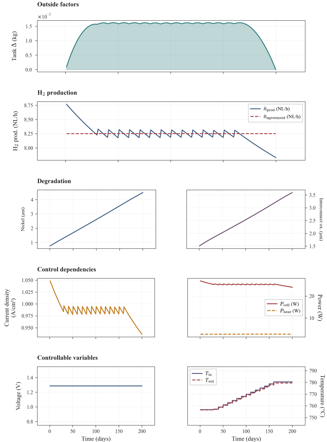
Figure 5.3: Constant-delivery optimum with free voltage and temperature controls ( N_t = 20 settings in Table 5.3). One corner case of a continuum of numerically equivalent local minima: after an initial potentiostatic-isothermal phase at the baseline optimum (Section 5.2), inlet temperature is raised in steps so that production tracks the contractual rate \dot{n}_{\text{H}_2, \text{agreement}} = 8.25 \text{ NL/h} (dashed pink line) while U remains fixed near 1.28 V. The tank inventory (left panel) builds to about 0.016 kg by day 40 and is then drawn down only in
