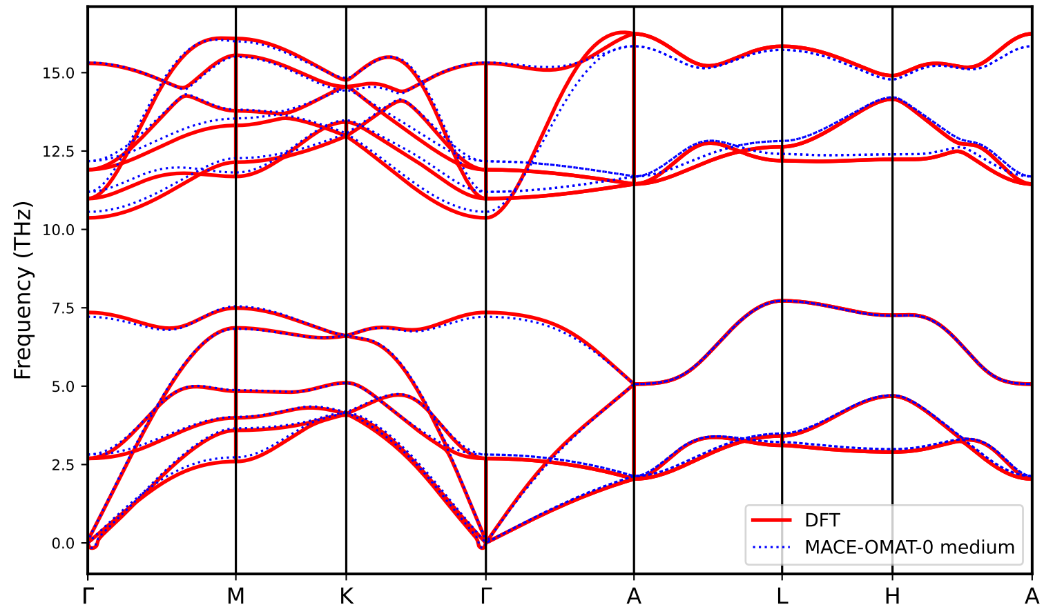
Phonon dispersion — DFT vs MACE-OMAT-0 medium
