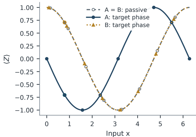
(a) Passive and phase responses
