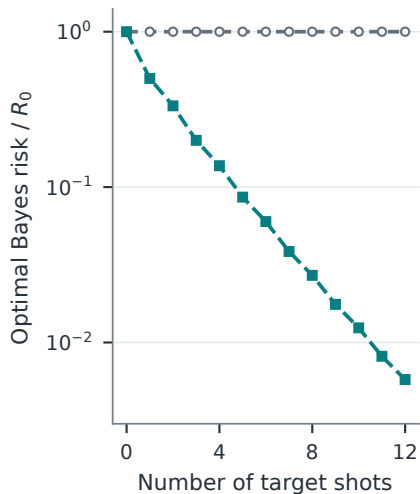
(b) Exact prediction risk
