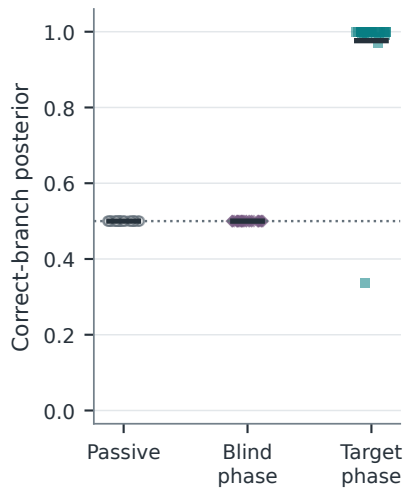
(c) Hidden-branch inference
