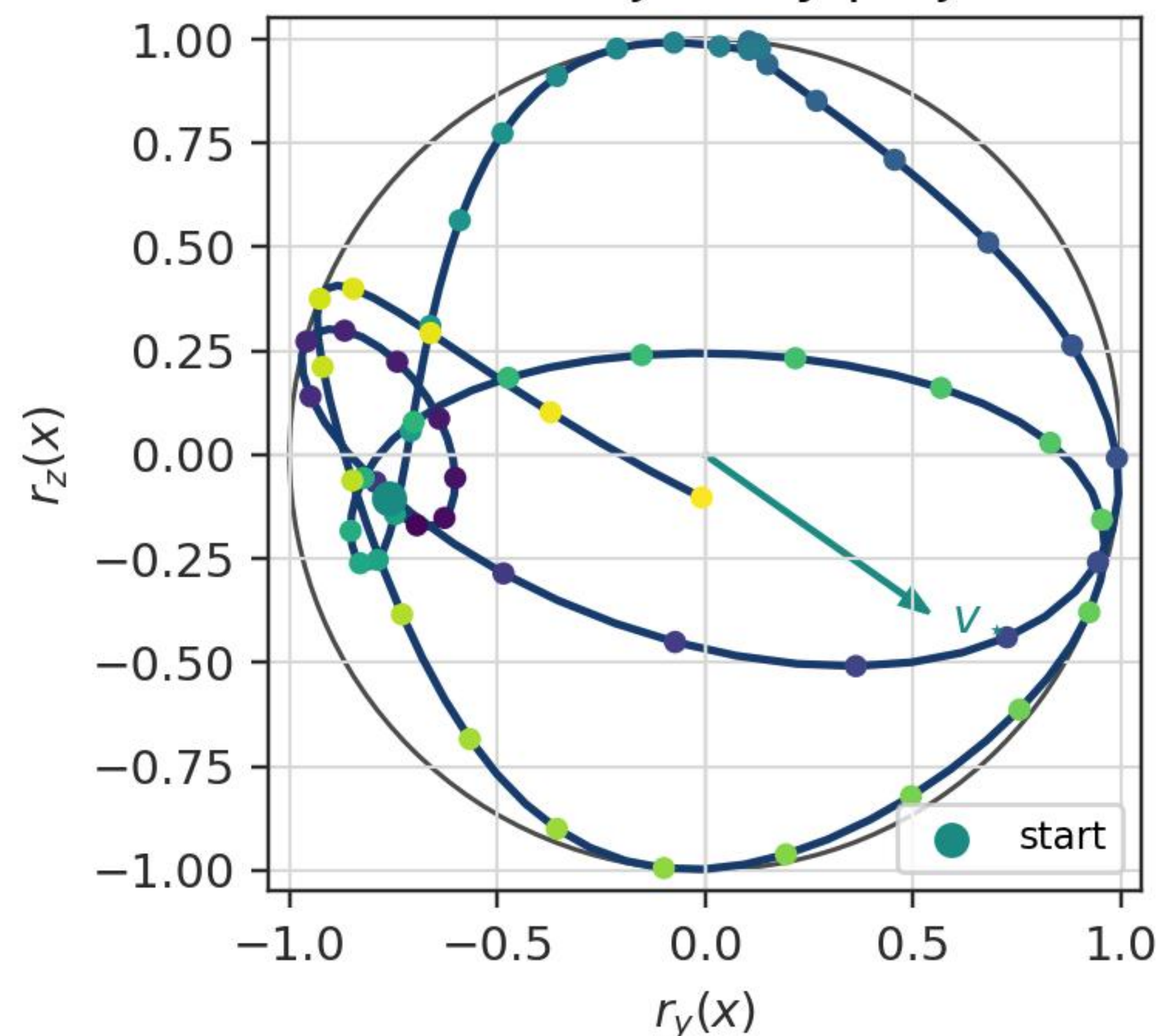
(b) Bloch trajectory projection
