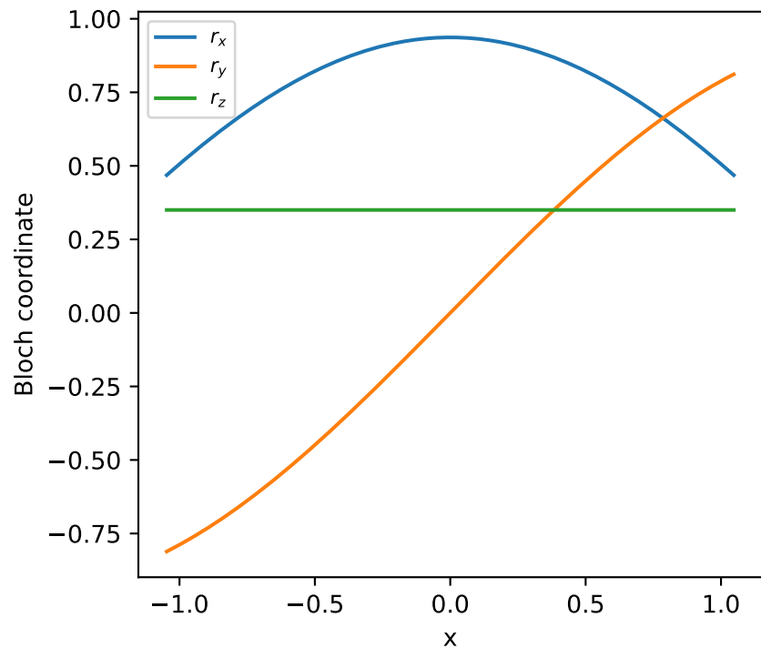
Observable state motion with constant \langle Z \rangle
