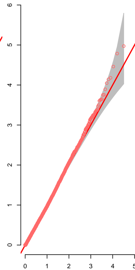
FarmCPU.FHBSPKINC
