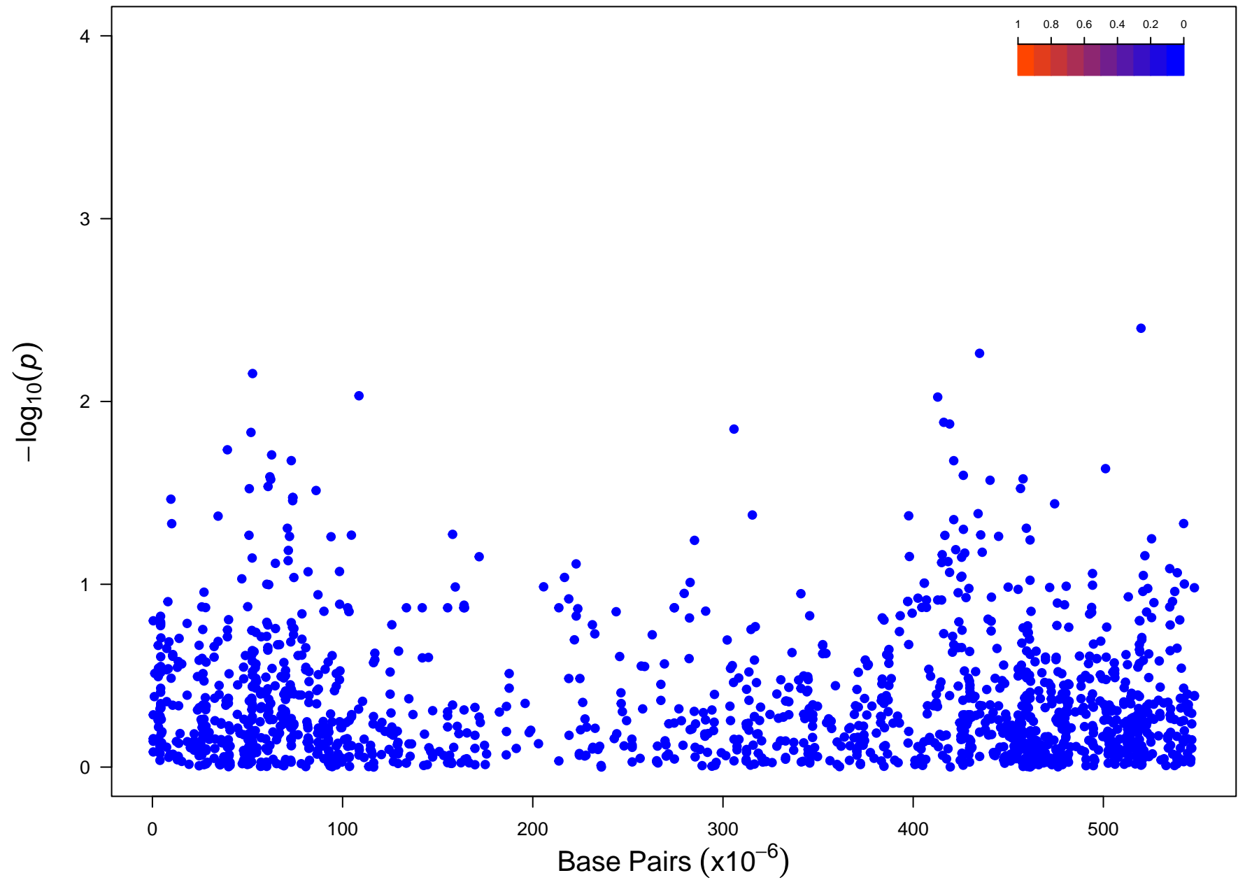
Chromosome 1
