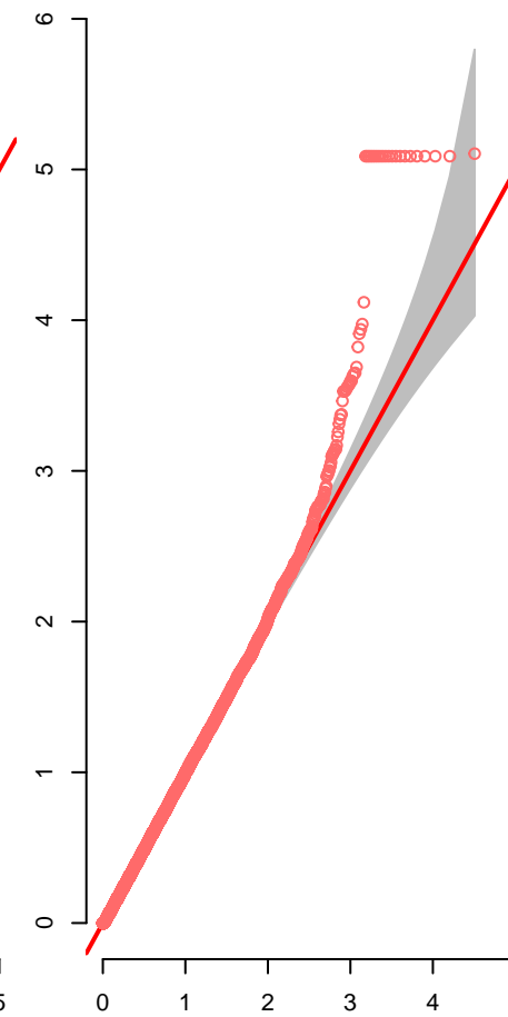
FarmCPU.PTHT
