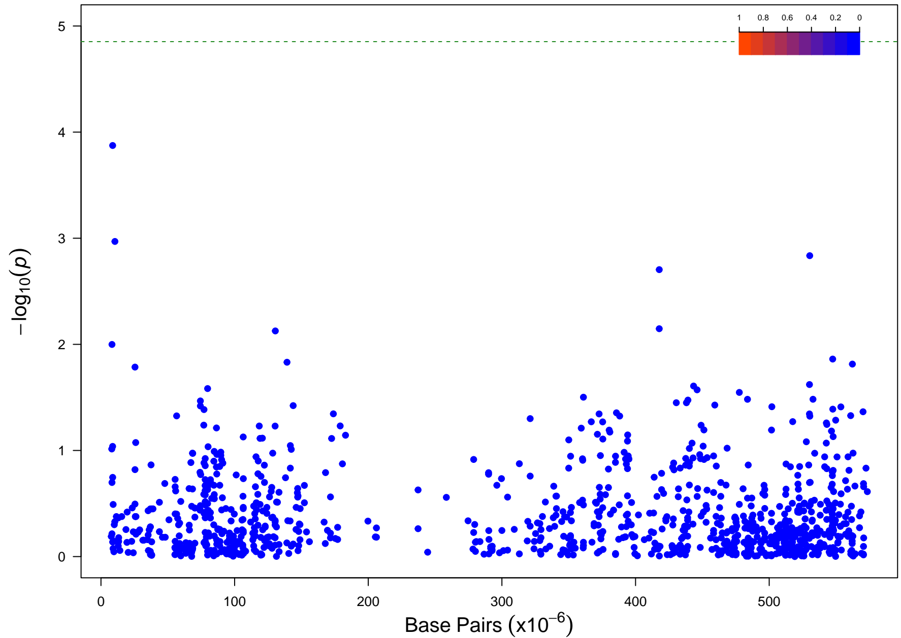
Chromosome 15
