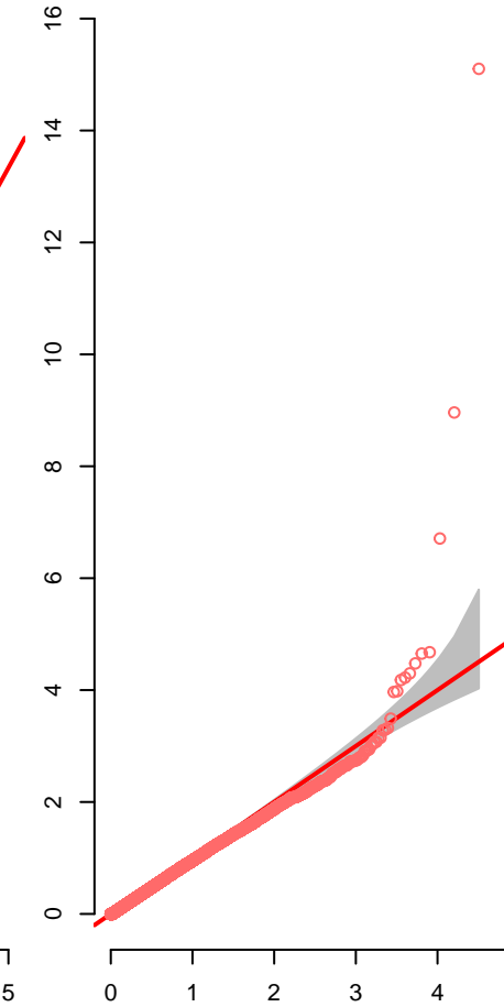
FarmCPU.ZDK
