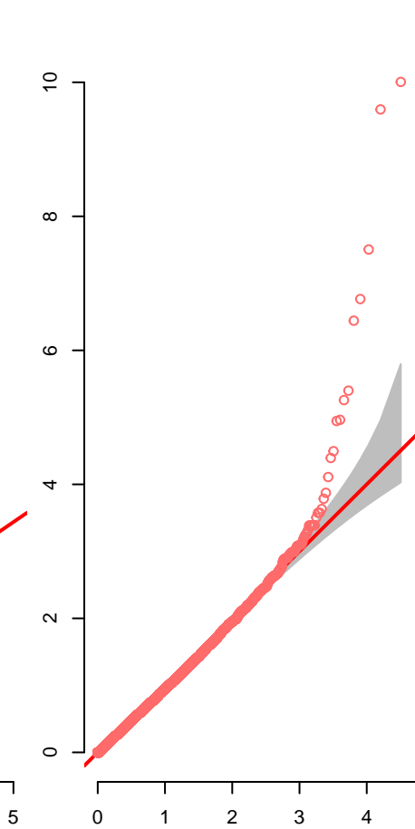
FarmCPU.BLSSEV
