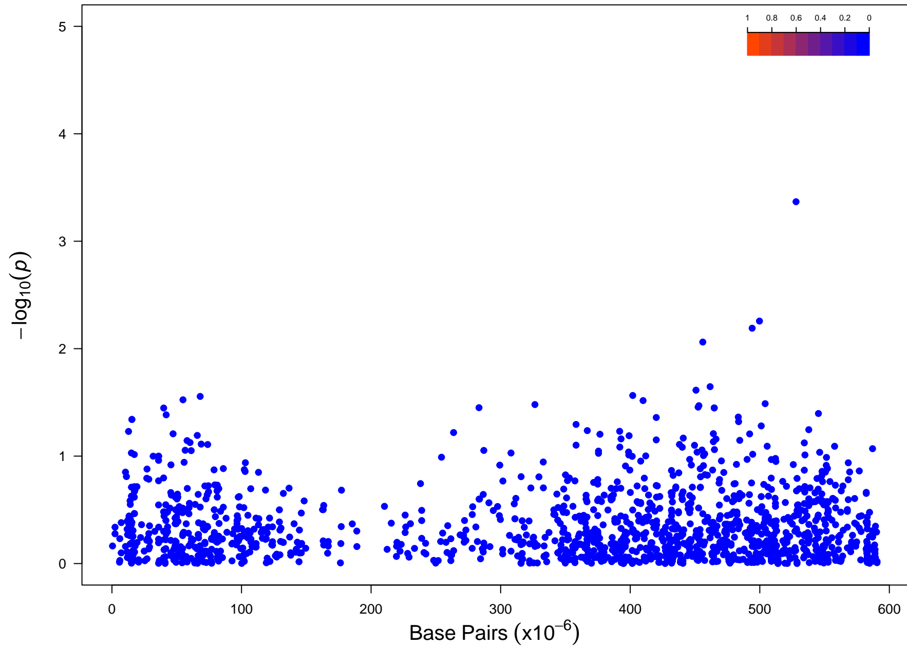
Chromosome 19
