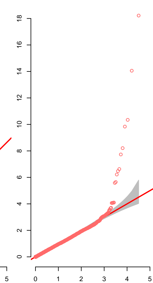
FarmCPU.HSATIVLSEV
