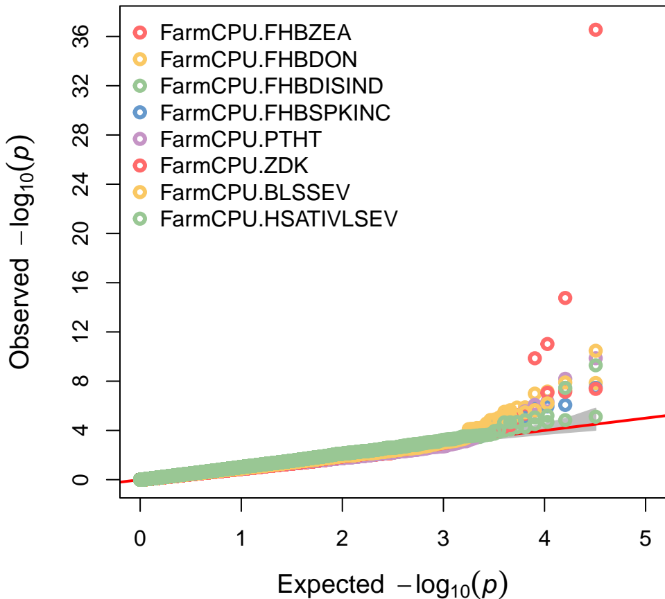
QQ plot
