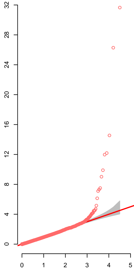
FarmCPU.FHBDON
