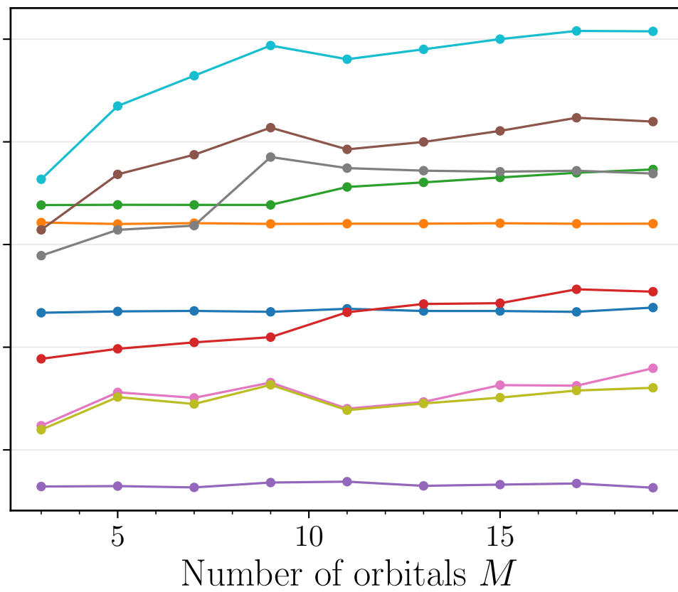
N = 3 electrons
