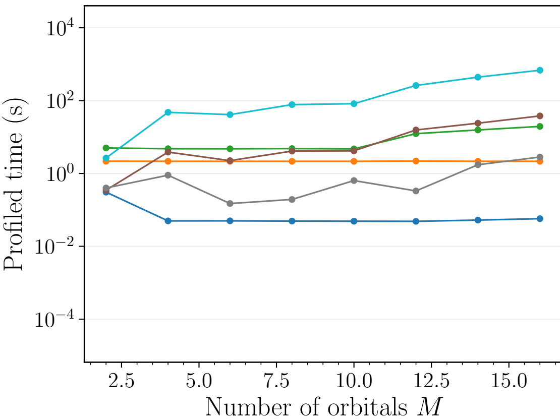
N = 2 electrons
