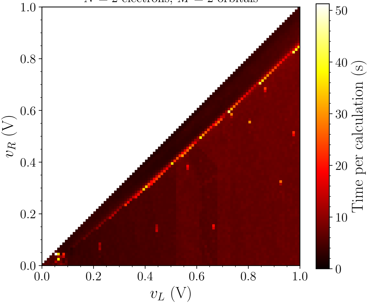
N = 2 electrons, M = 2 orbitals
