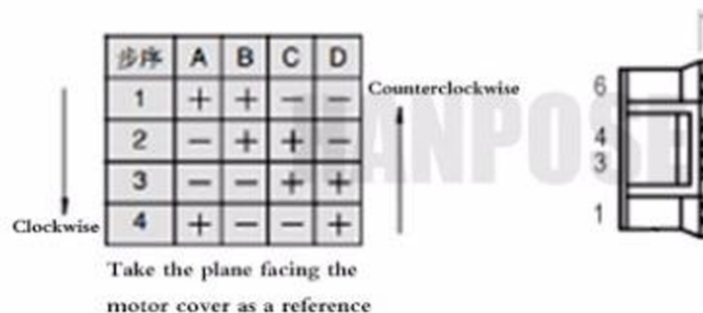
Wiring sequence
