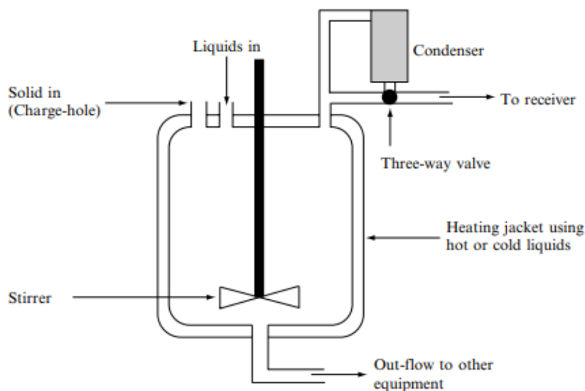
Figure SC-H&M-TRB - 28: A diagrammatic representation of a typical reaction vessel. The three-way valve enables the condenser to be used to either reflux or distil the liquids in the reaction vessel.
