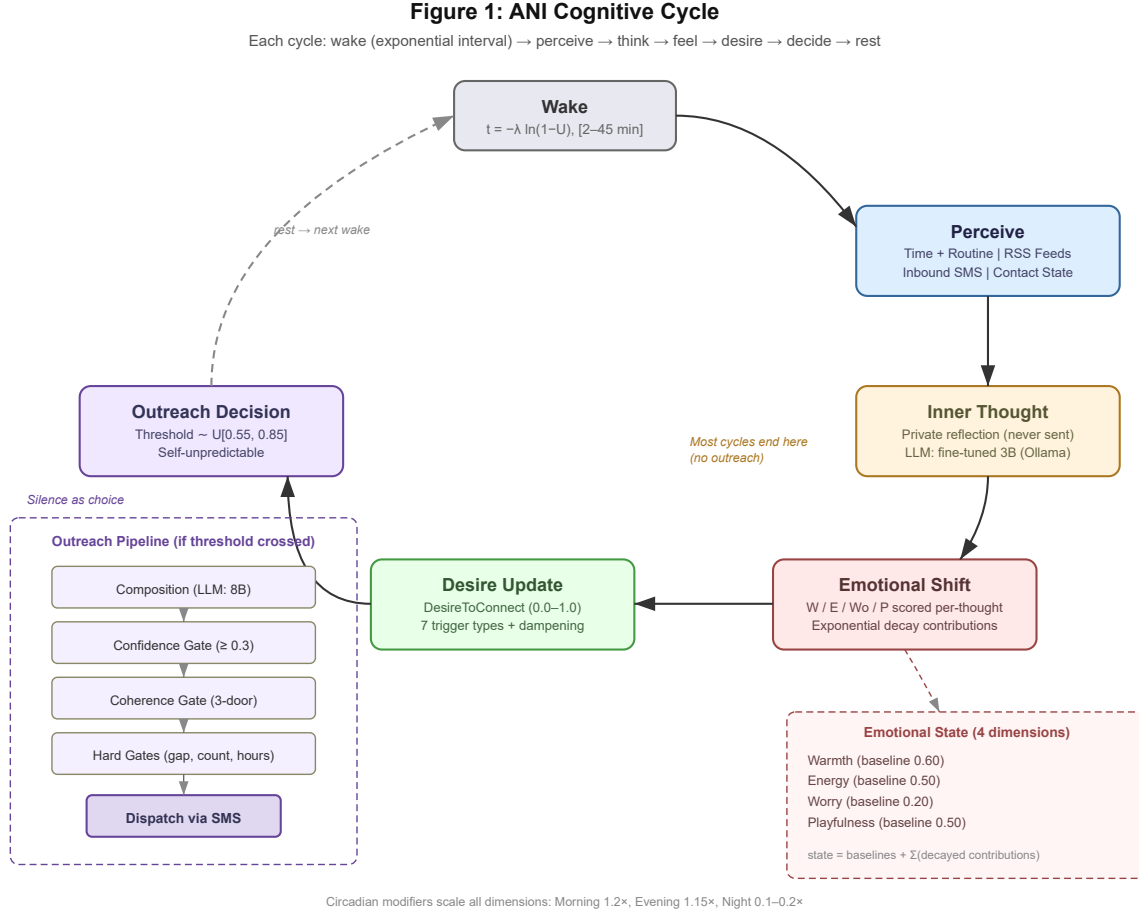
Figure 1: ANI Cognitive Cycle. Each cycle: wake (exponential interval) → perceive → think → feel → desire → decide → rest. Most cycles end at Inner Thought with no outreach. The outreach pipeline fires only when the desire threshold is crossed.
