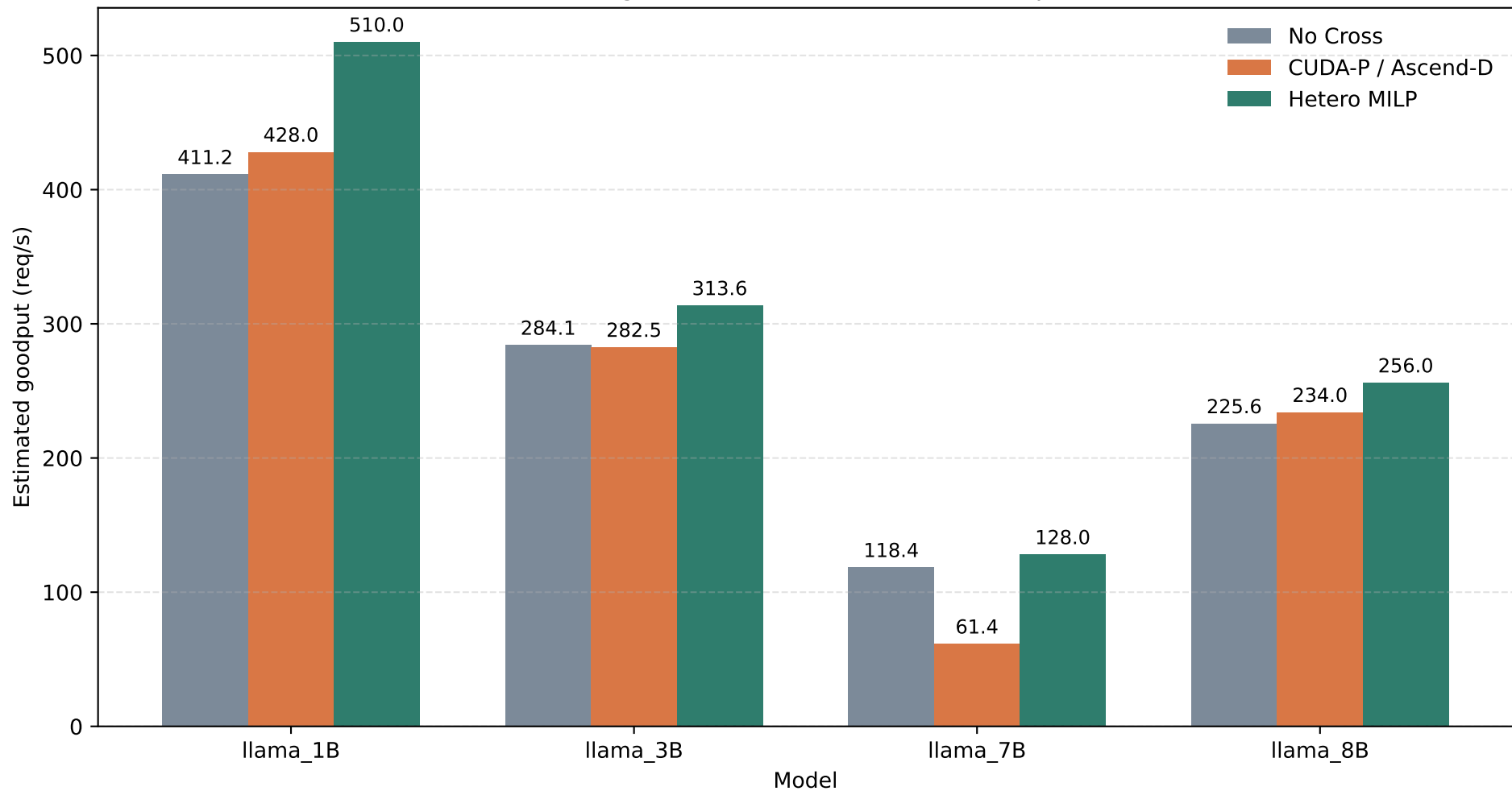
Heterogeneous DistServe Search Goodput
