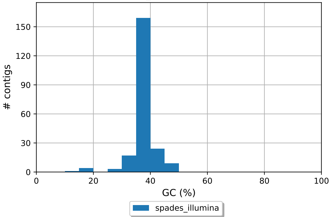
spades_illumina GC content
