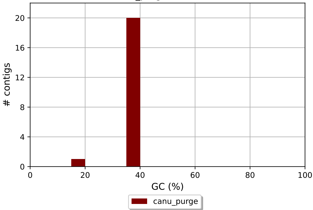
canu_purge GC content
