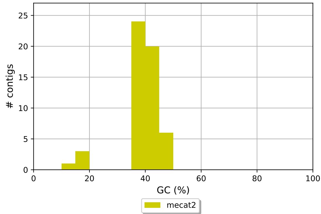
mecat2 GC content
