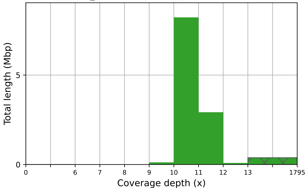
spades_hifi coverage histogram (bin size: 1x)
