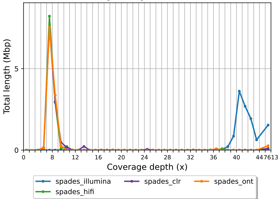
Coverage histogram (bin size: 1x)
