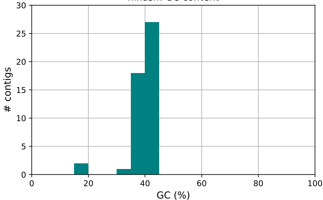
hifiasm GC content
