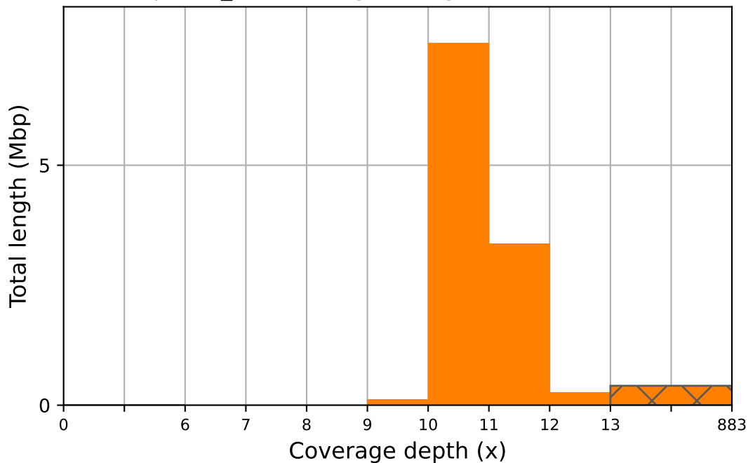
spades_ont coverage histogram (bin size: 1x)
