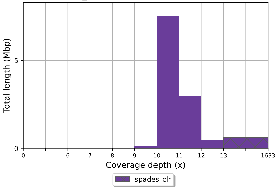
spades_clr coverage histogram (bin size: 1x)
