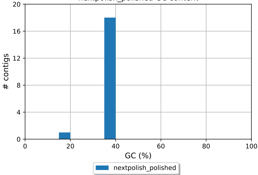
nextpolish_polished GC content
