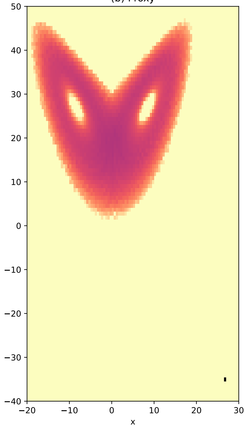
(b) Proxy
