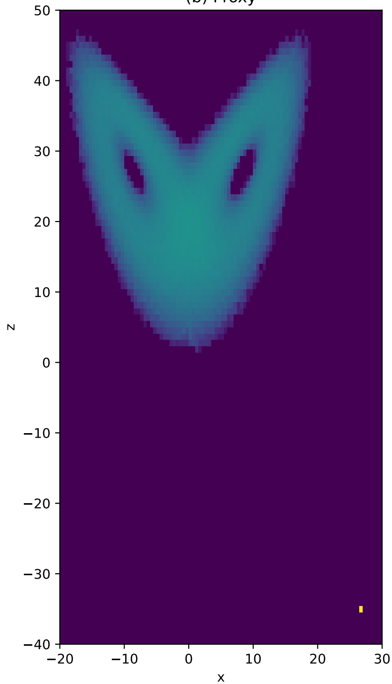
(b) Proxy
